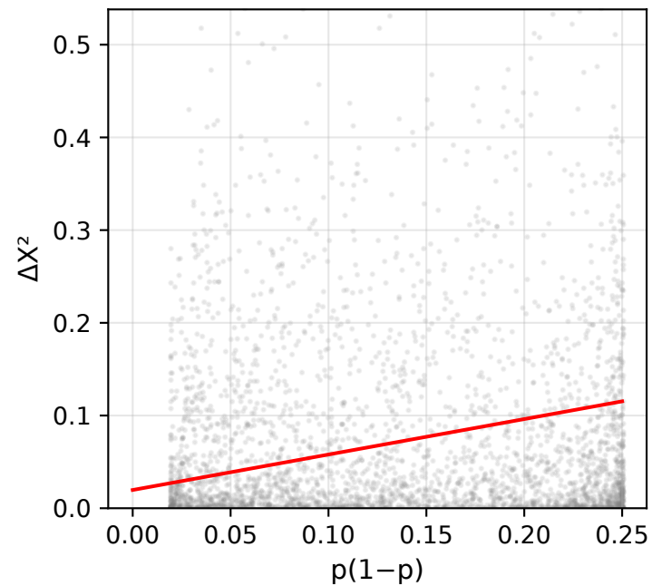
4. Boundary scaling (slope=0.382)
