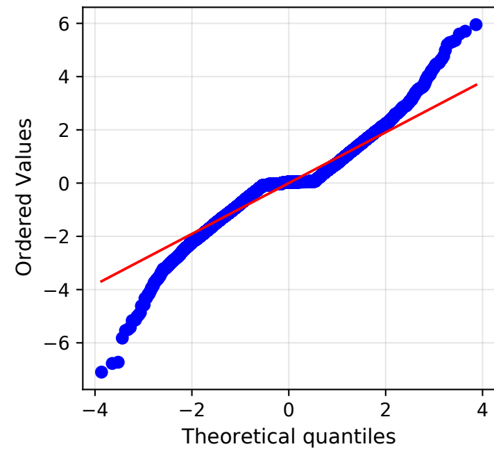
1. Q-Q (std. increments vs Normal)
