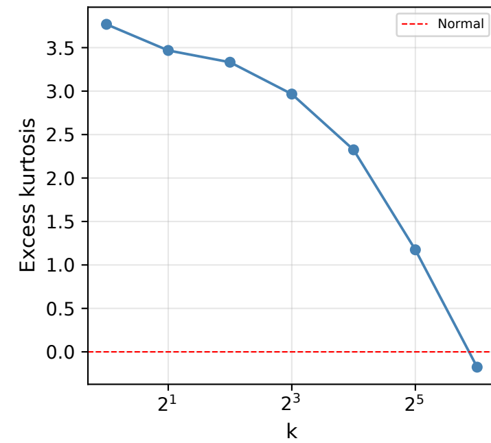
3. Kurtosis vs aggregation scale k
