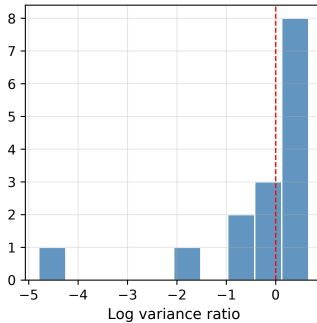
5. \log(\text{Var}_{\text{last}}/\text{Var}_{\text{first}}) per contract
