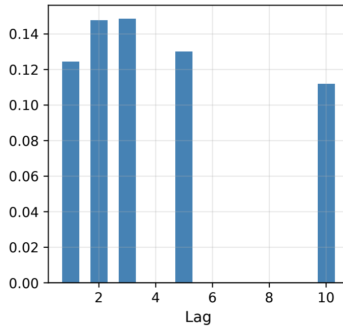
2. Mean ACF( \Delta X^2 ) across contracts
