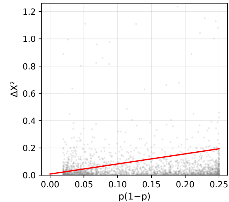
4. Boundary scaling (slope=0.740)
