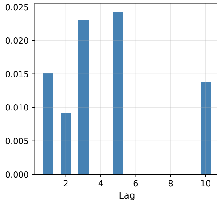
2. Mean ACF( \Delta X^2 ) across contracts
