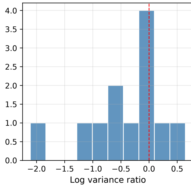
5. \log(\text{Var\_last}/\text{Var\_first}) per contract
