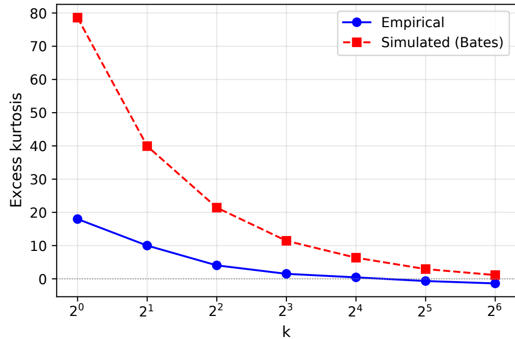
§4.7 Aggregational Gaussianity
