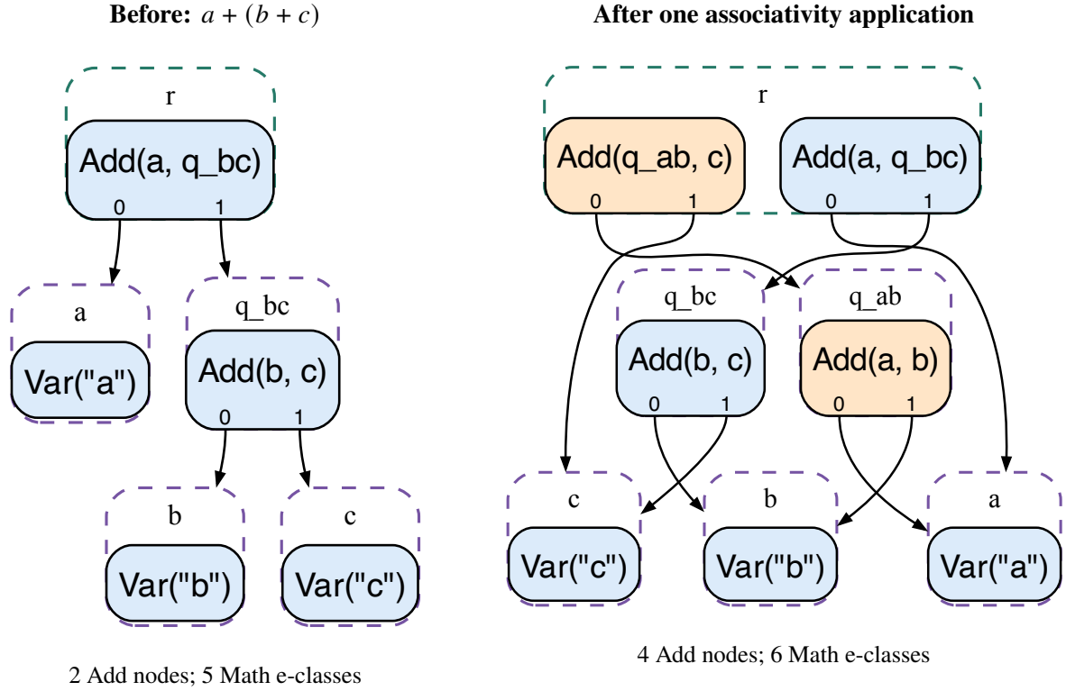
Figure 4: Read the change from left to right. Native egglog introduces \text{Add}(a, b) and \text{Add}(q_{ab}, c) (orange) and unions the latter with the existing root r . Blue nodes were already present. Dashed enclosures are native e-classes; numbered ports are argument positions, and arrows terminate at child classes. Both graphs come from executable prefixes of math-mini-trace.egg , through egglog’s own DOT exporter. Var ’s String payloads are inlined into its label.
