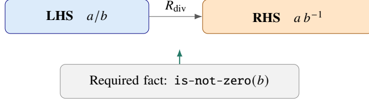
Figure 5: Why a binding is not enough. The guarded division rule is copied from math.egg : a native check confirms that it does not apply without is-not-zero(b) and applies after that fact is supplied. This illustrates an external obligation; it does not independently establish that the supplied mathematical assertion is true.
