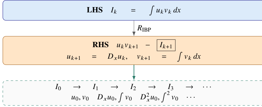
Figure 15: A productive infi rule composition from the actual IBP rule. In the IBP-only fragment, the boxed residual regenerates the same pattern with strictly deeper Diff/Integral arguments. Four native steps yield 11, 17, 23, and 29 Math e-nodes. The all-depth argument requires the restricted theory; full math.egg may simplify the derivative and terminate this family.
