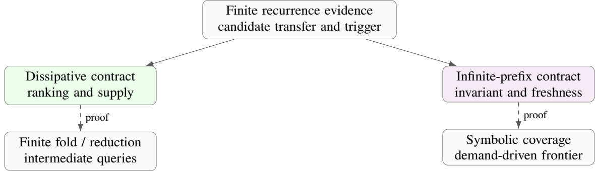
Figure 17: Proof obligations separate observed regularity from summary-based execution. A finite witness is not a certificate of either termination or unbounded generation.
