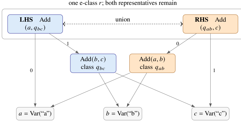
Figure 3: One native application of Add associativity from math.egg . The matched a + (b + c) is retained and the constructed (a + b) + c joins its class. q_{ab} and q_{bc} are separate child e-classes; argument order is explicit in the node labels. Primitive String values below Var nodes are omitted.
