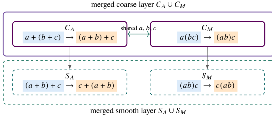
Figure 9: CCSS with real Add/Mul rules from math.egg . Both input trees are declared initially and share a, b, c ; there is no S-to-C dependency. The restricted native fragment saturates to 12 Add and 12 Mul rows. Layer outlines indicate regrouping, not deletion of the four original compositions.
