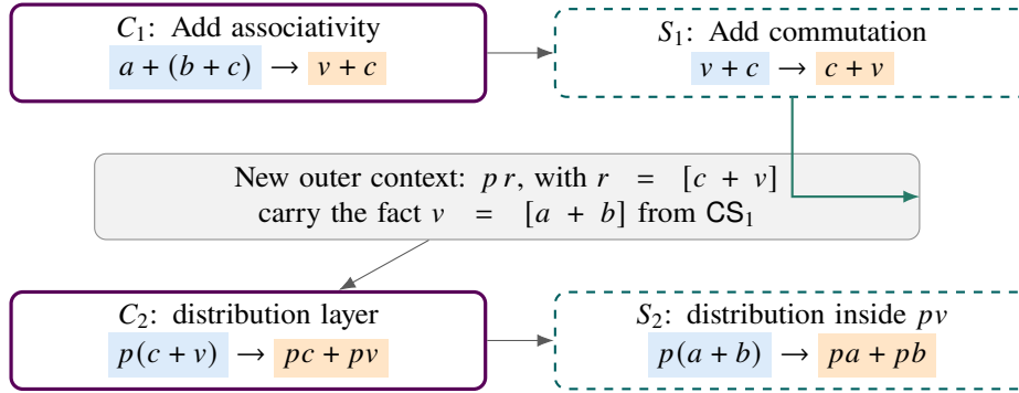
Figure 7: A native-checked CSCS example using associativity, commutation, and distribution from math.egg . Distribution may match several retained representatives; one is shown. The declared interface of CS_2 carries the \text{Add}(a, b) fact, so its inner distribution step does not fetch it for free. The fresh outer multiplication context is supplied only after CS_1 .
