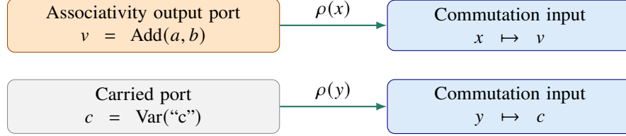
Figure 4: A concrete relative binding from the native Add trace: the next rule matches \text{Add}(v, c) , so its formal variables become x = v and y = c . This is a port map, not addition of numeric binding offsets. The producer-to-consumer row witness is recorded in the evidence file.
