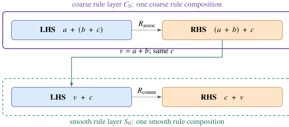
Figure 6: A concrete CS unit from math.egg . The first step requires the external entry Add(a, Add(b, c)) ; the second reads the associativity output and needs no new external fact. The repeated orange/blue expression is one reused node, shown in two occurrence roles, not duplicated storage. Labels C_0, S_0 describe this selected interface, not globally unique runtime layer IDs.
