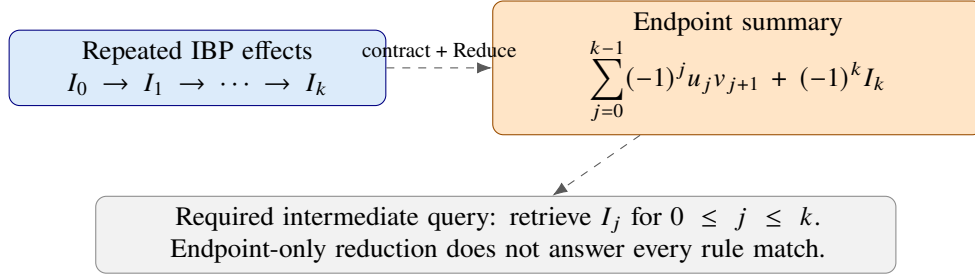
Figure 16: How an infi composition could feed ripen: summarize the alternating endpoint, but retain an indexed residual interface. This is a proposed contract for the worked IBP family with additional exact additive laws, not a claim that the current Reduce DSL automatically discovers or executes this alternating-sum summary.
