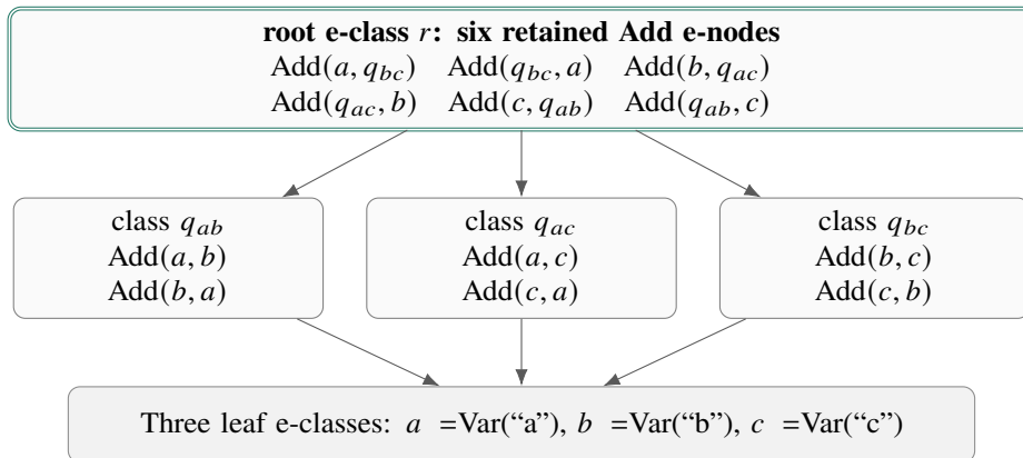
Figure 10: The retained body of a saturated rule composition in the native Add fragment: 12 Add rows and three Var rows in seven Math e-classes. Grouped arrows summarize child-class references; the row labels preserve argument order. This is saturation under the selected associativity/commutation theory, not under all of math.egg . Trigger and binding data belong to the composition too.
