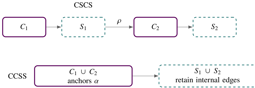
Figure 9: CSCS preserves a cross-unit dependency. CCSS regroupes C and S only under its contract. Neither operation removes external-input obligations.
