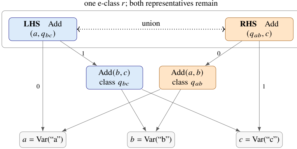
Figure 4: One native application of Add associativity from math.egg . The matched a + (b + c) is retained and the constructed (a + b) + c joins its class. q_{ab} and q_{bc} are separate child e-classes; argument order is explicit in the node labels. Primitive String values below Var nodes are omitted.
