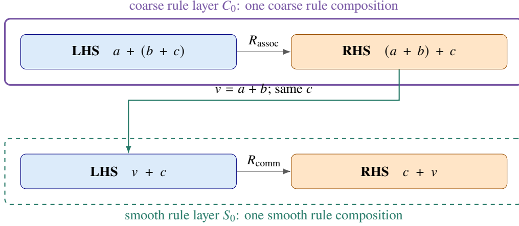
Figure 7: A concrete CS unit from math.egg . The first step requires the external entry Add(a, Add(b, c)) ; the second reads the associativity output and needs no new external fact. The repeated orange/blue expression is one reused node, shown in two occurrence roles, not duplicated storage. Labels C_0, S_0 describe this selected interface, not globally unique runtime layer IDs.
