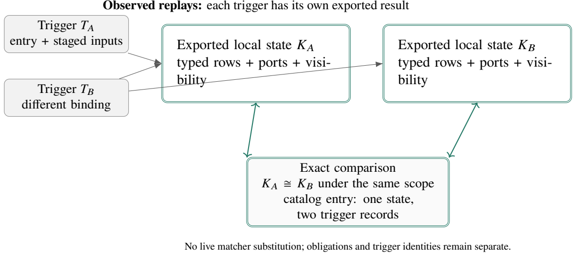
Figure 3: What the implementation actually shares. The baseline is two separately replayed trigger instances with exported local states. The catalog may group the states after exact typed graph comparison, while retaining both trigger contracts. This is the semantic distinction that a pipeline box alone cannot show: the shared object is an exported description, not a new tier0 rule or a deleted history.
