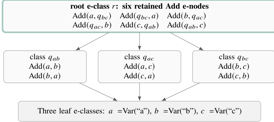
Figure 11: The retained body of a saturated rule composition in the native Add fragment: 12 Add rows and three Var rows in seven Math e-classes. Grouped arrows summarize child-class references; the row labels preserve argument order. This is saturation under the selected associativity/commutation theory, not under all of math.egg . Trigger and binding data belong to the composition too.
