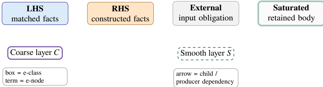
Figure 2: Visual vocabulary. Fill identifies the role of facts in a rule application; outline identifies the containing layer. LHS/RHS labels and solid/dashed outlines also distinguish the roles without color. A box with several terms is an e-class; the terms inside it are e-nodes, and arrows name the child or producer relation. An e-node may be an RHS in one step and an LHS in the next.
