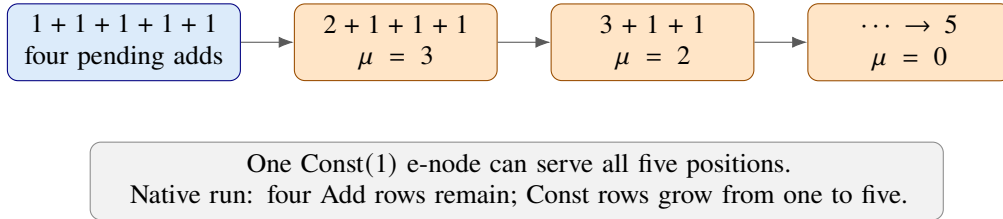
Figure 14: A dissipative composition using the native constant-fold rule from math.egg . The initial expression is left-associated; outer Add facts are part of the declared entry. The remaining work frontier decreases, not the stored fact set. No pruning is enabled in this example.
