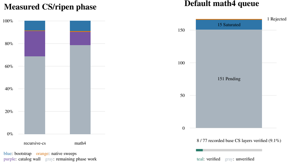
Figure 20: Recent bounded native observations. The left panel uses disjoint portions of the measured phase from five-run medians: bootstrap, native sweeps, catalog wall, and remaining phase work. Catalog wall includes catalog I/O and grouping; exact graph comparison alone was 0.58% of recursive-cs and 1.08% of math4. The right panel is the default four-round math4 queue: 15 Saturated, 1 Rejected, and 151 Pending candidates, with 8 of 77 recorded base CS layers verified. These are bounded experiments; Pending is not a negative result, and the coverage denominator is the recorded base-CS population, not every possible layer or the live tier0 graph.
