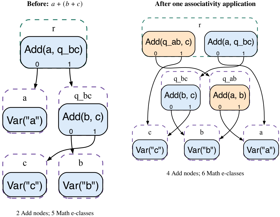
Figure 4: Read the change from left to right. Native egglog introduces \text{Add}(a, b) and \text{Add}(q_{ab}, c) (orange) and unions the latter with the existing root r . Blue nodes were already present. Dashed enclosures are native e-classes; numbered ports are argument positions, and arrows terminate at child classes. Both graphs come from executable prefixes of math-mini-trace.egg , through egglog's own DOT exporter. Var 's String payloads are inlined into its label.
