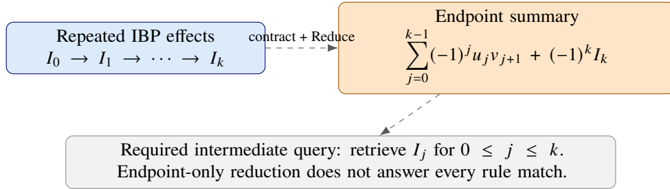
Figure 18: How an infi composition could feed ripen: summarize the alternating endpoint, but retain an indexed residual interface. This is a proposed contract for the worked IBP family with additional exact additive laws, not a claim that the current Reduce DSL automatically discovers or executes this alternating-sum summary.
