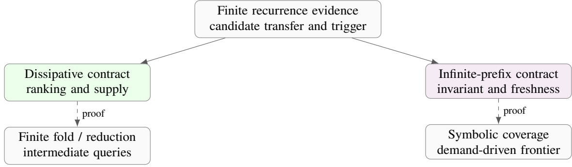
Figure 19: Proof obligations separate observed regularity from summary-based execution. A finite witness is not a certificate of either termination or unbounded generation.
