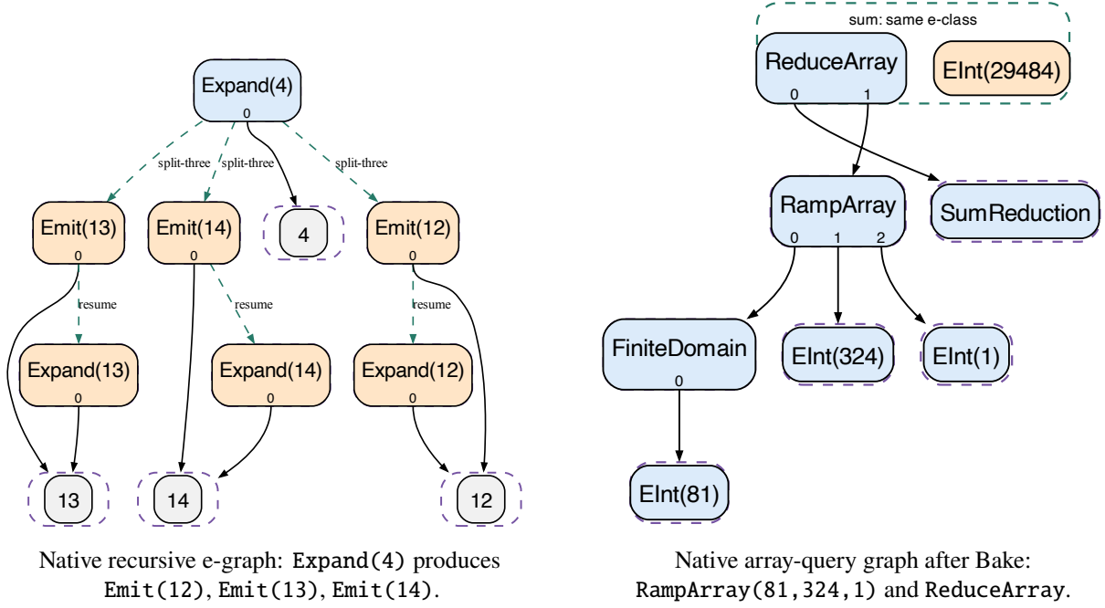
Figure 17: The recursive-array case in two stages. The left graph is an executable Math e-graph snapshot; solid edges are native child references and dashed split-three / resume edges are explicitly labelled rule-instance annotations. The right graph is the native tier2 array query produced from the certified Bake law. Its paper annotation removes helper arithmetic alternatives, but the remaining nodes and solid child-class edges are checked against the native DOT export.
