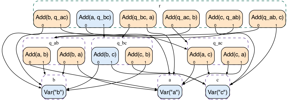
Figure 11: The Add body exported by the mini.math.egg fragment. This figure is generated from egglog 's own -to-dot serializer: dashed clusters are e-classes, solid boxes are e-nodes, and numbered ports preserve ordered child positions. The paper-side transformation only inlines Var string payloads and annotates the entry-relative colours; it checks that every Math node and ordered child edge from the native DOT survives. The graph has 12 Add nodes, three Var nodes, and seven Math e-classes.
