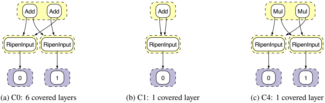
Figure 21: Top three exact saturated bodies in the default four-round math capture, ranked by distinct covered CS layers. Dashed rounded regions are e-classes; constructor boxes and ordered child ports are emitted by egglog’s native EGraph serializer. C0 and C1 are Add bodies with different boundary aliasing; C4 is a Mul body. The corresponding .dot and .svg files are retained beside the paper figure.
