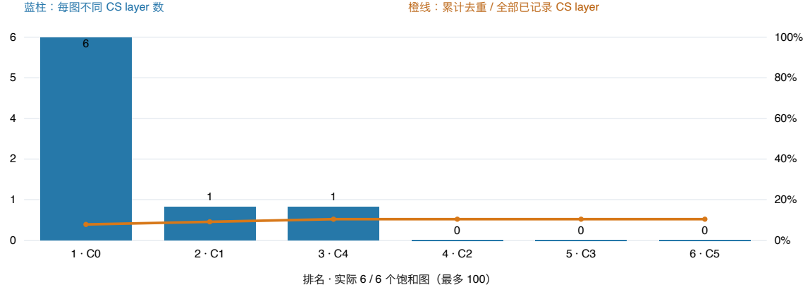
Figure 20: Ripen reuse coverage from the default math4 run introduced in commit a4e148e . Each blue bar is one SaturatedRuleComposition body, ranked by the number of distinct base CS layers whose complete member set reached exact saturation equality. The orange line is cumulative coverage after de-duplicating layer IDs across bodies. The run has six catalogued bodies, eight verified layers out of 77 recorded base CS layers (10.4%), six unattributed triggers, and queue states 15 Saturated, 1 Rejected, and 151 Pending. Pending layers remain unknown; this is a provenance-backed reuse lower bound, not a tier0 replacement rate or a storage-compression measurement.
