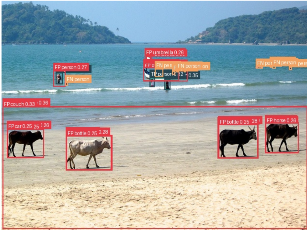
图 4: Per-class false positive case
