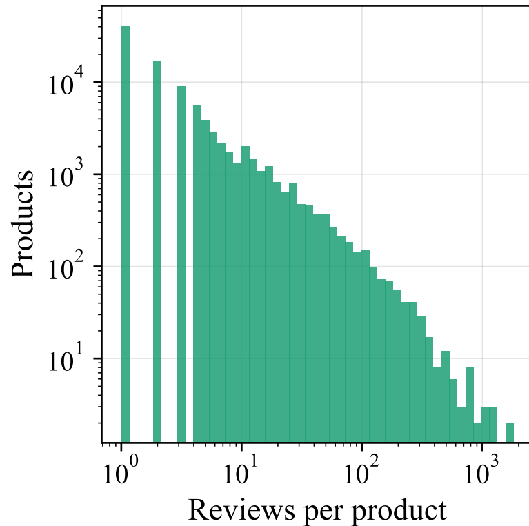
(b) Product coverage (log-log)
