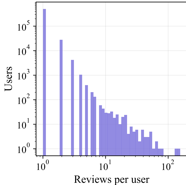
(c) User activity (log-log)
