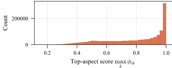
(a) Aspect-concentration per review
