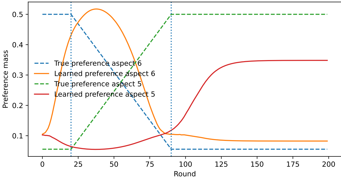
Aspect-level preference drift tracking: GUMBEL
