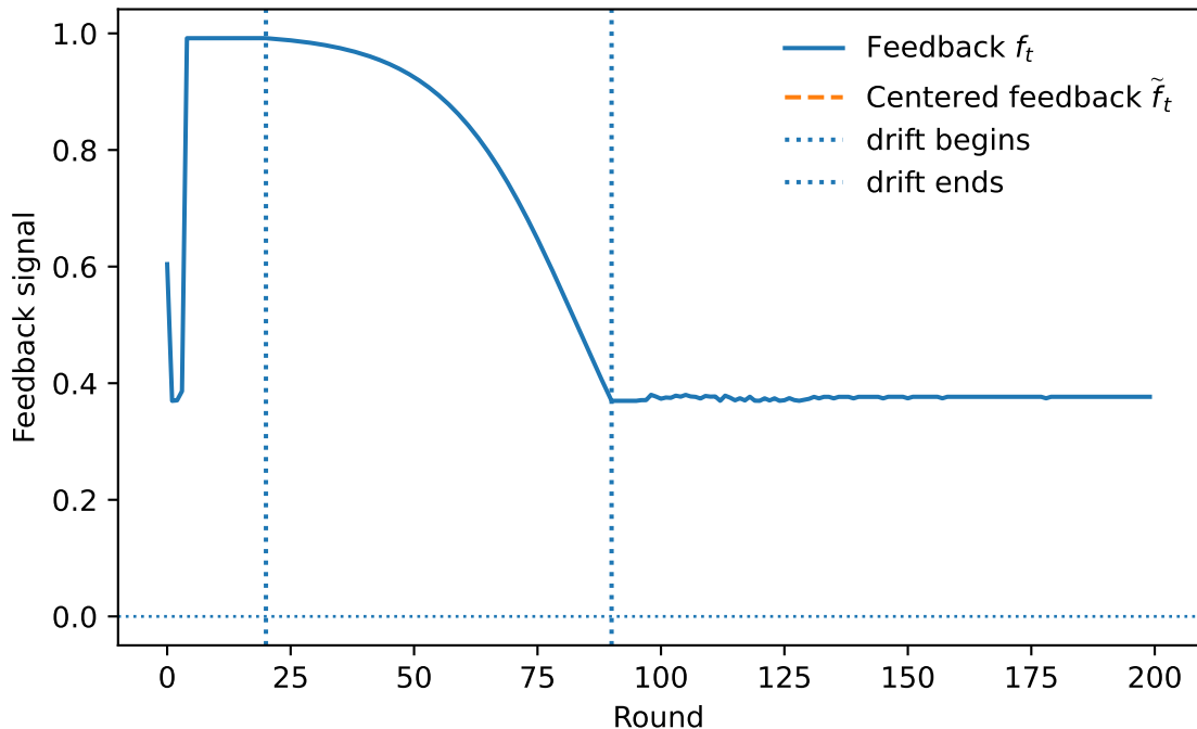
PREFER-MMR: feedback under drift
