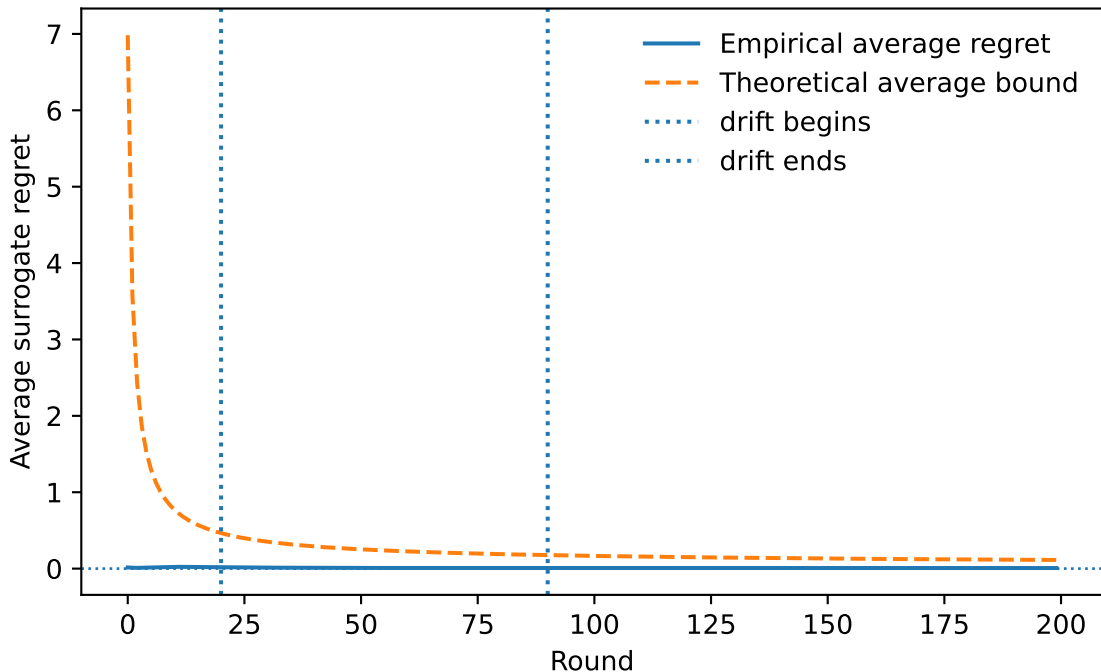
PREFER-GUMBEL: average regret under drift
