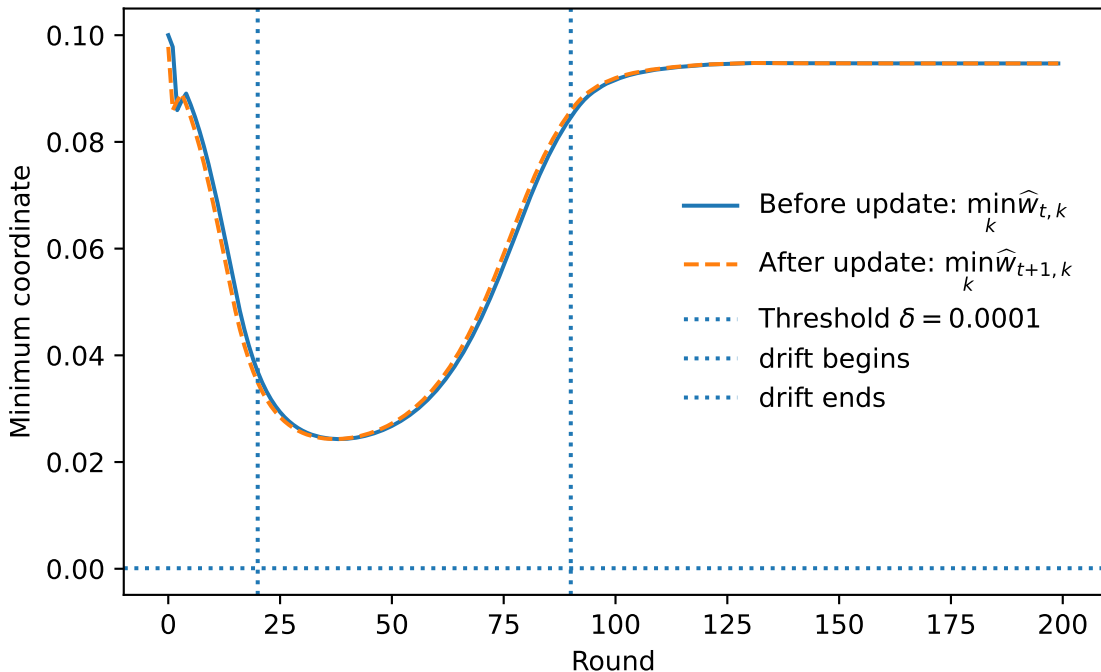
PREFER-MMR: truncated-simplex check under drift
