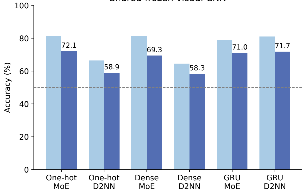
Shared frozen visual CNN
