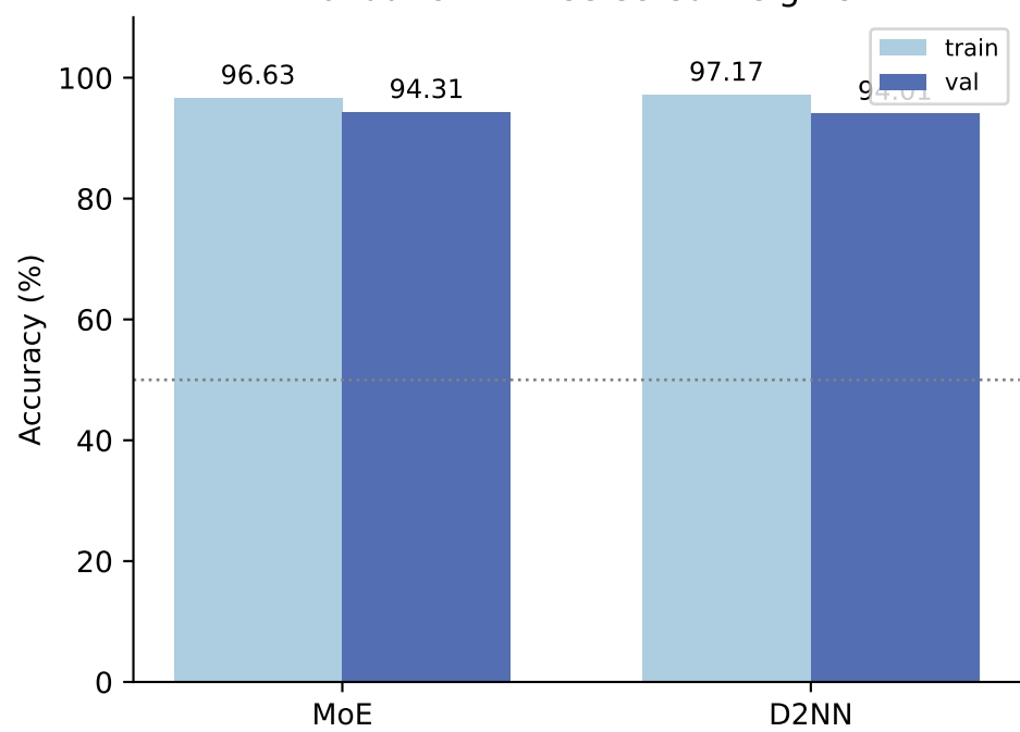
Validation-NLL-selected weights
