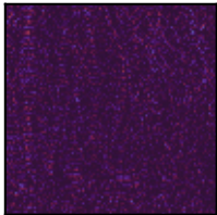
Language · expert 2
