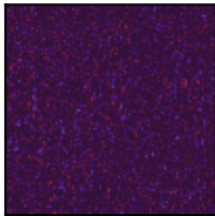
Vision · expert 0
