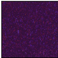
Vision · expert 3
