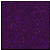
Vision · expert 1
