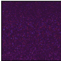
Language · expert 1
