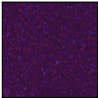
Vision · expert 2
