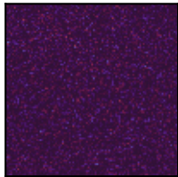
Language · expert 0
