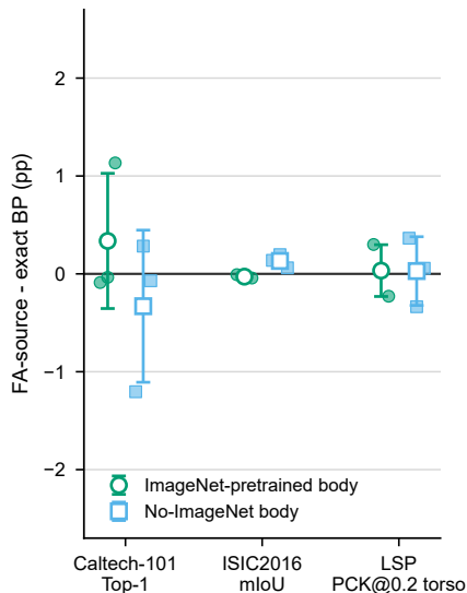
c Fixed source feedback tracks exact BP
