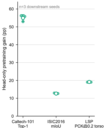
b ImageNet body improves head-only transfer
