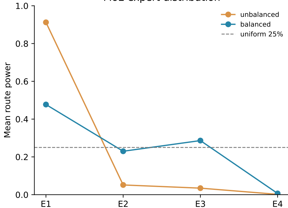
MoE expert distribution
