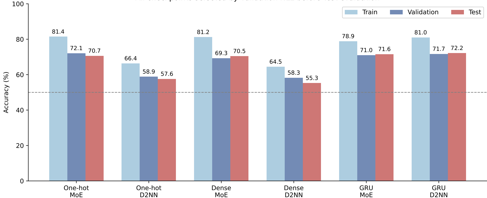
Shared frozen visual CNN | 2 layers + per-layer OEO | seed 17 All checkpoints selected by validation NLL before test evaluation
