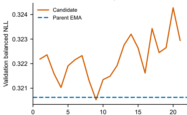
lowlr · rejected
