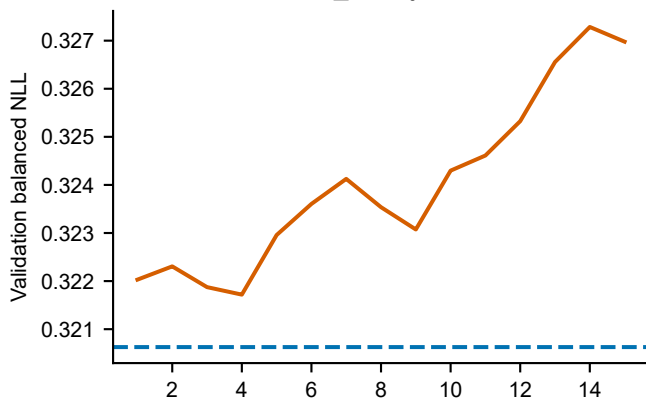
lowlr_ls · rejected
