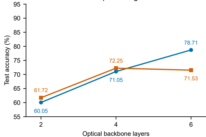
30-epoch budget
