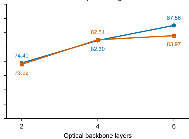
100-epoch budget
