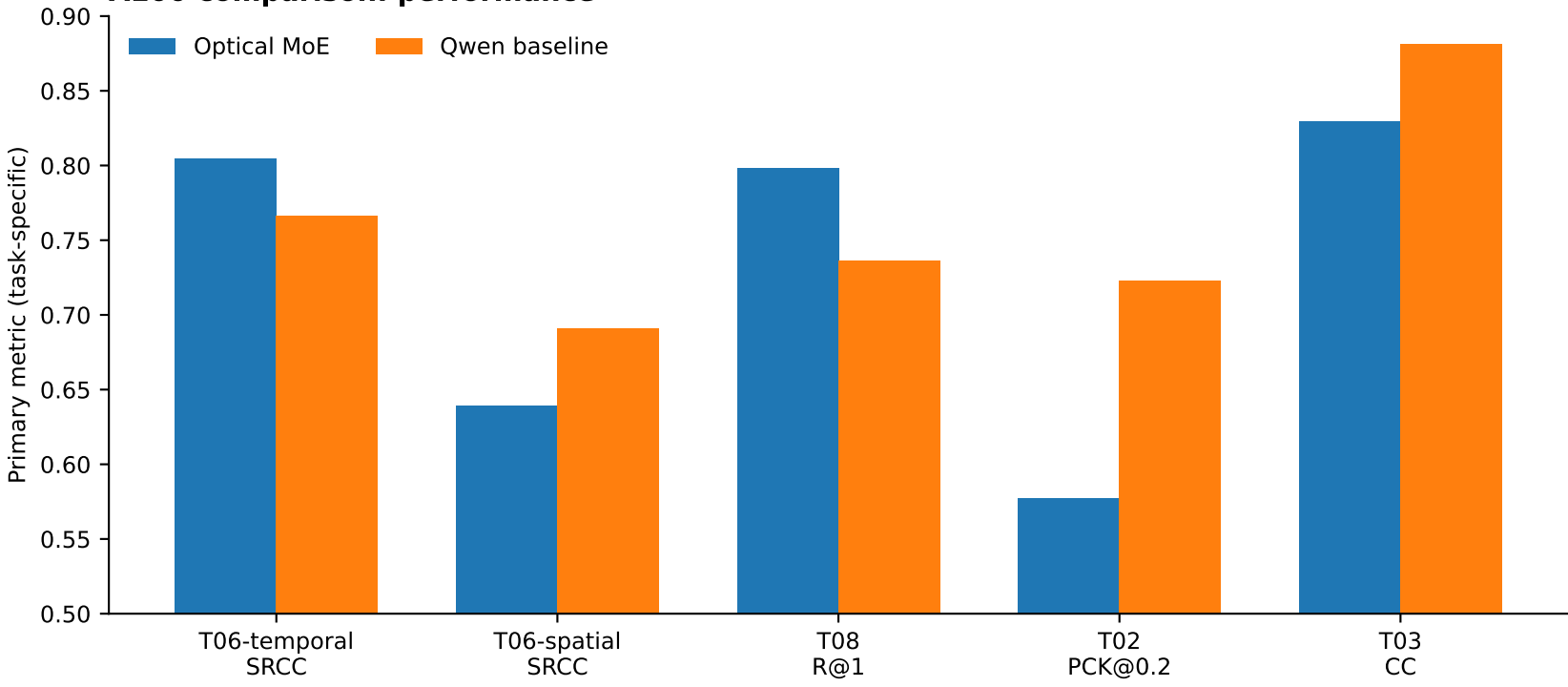
A100 comparison: performance
