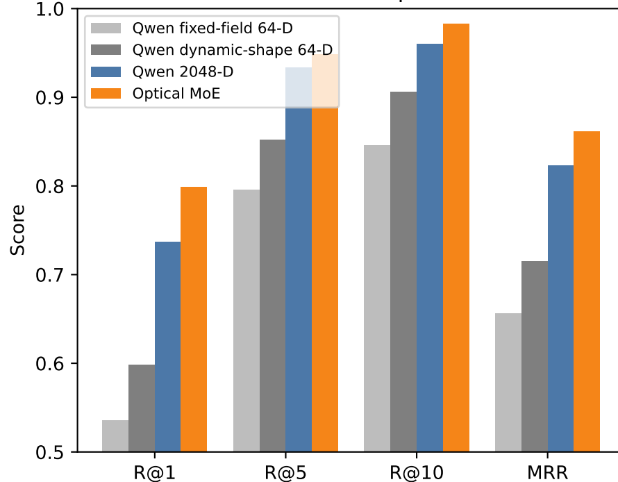
b Best checkpoint
