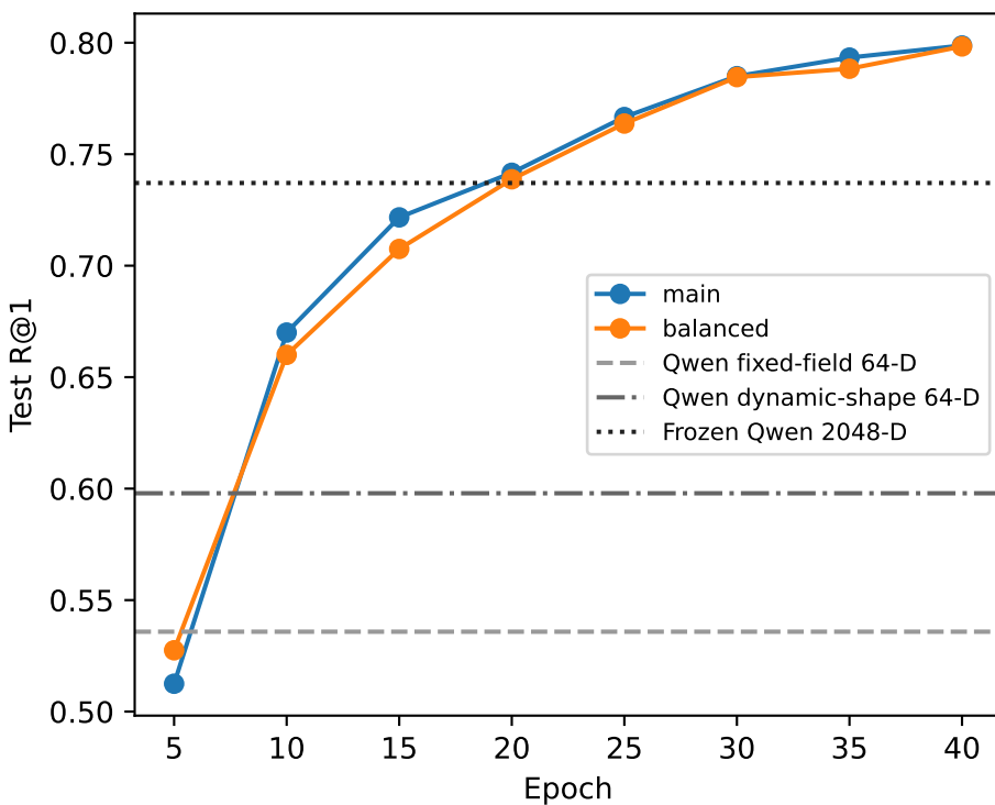
a Periodic test retrieval
