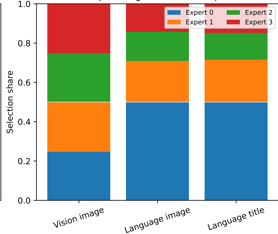
c Top-2 usage at selected epoch
