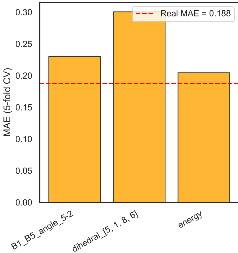
Per-feature shuffle test: MAE (lower is better)
