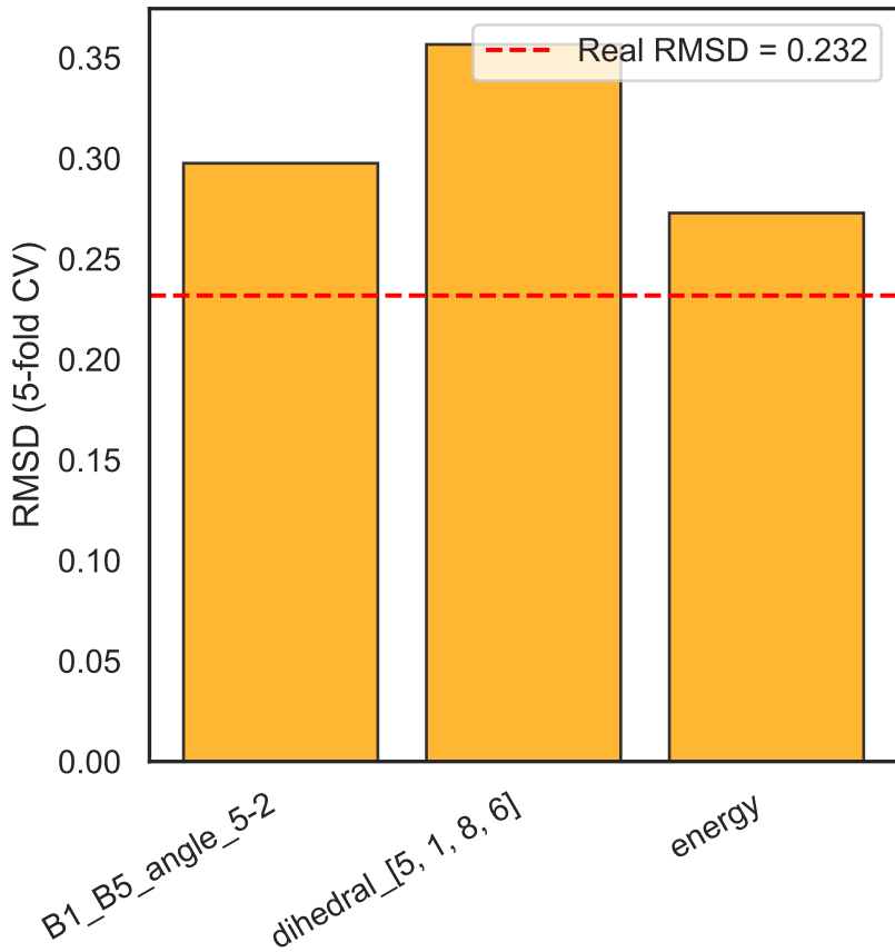
Per-feature shuffle test: RMSD (lower is better)
