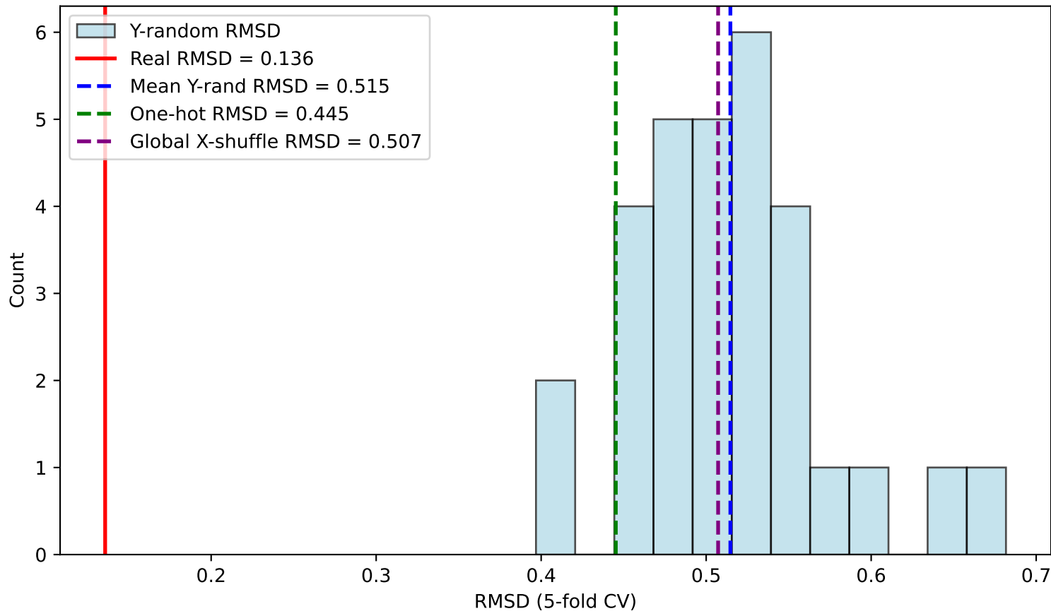
Validation (lower is better): RMSD
