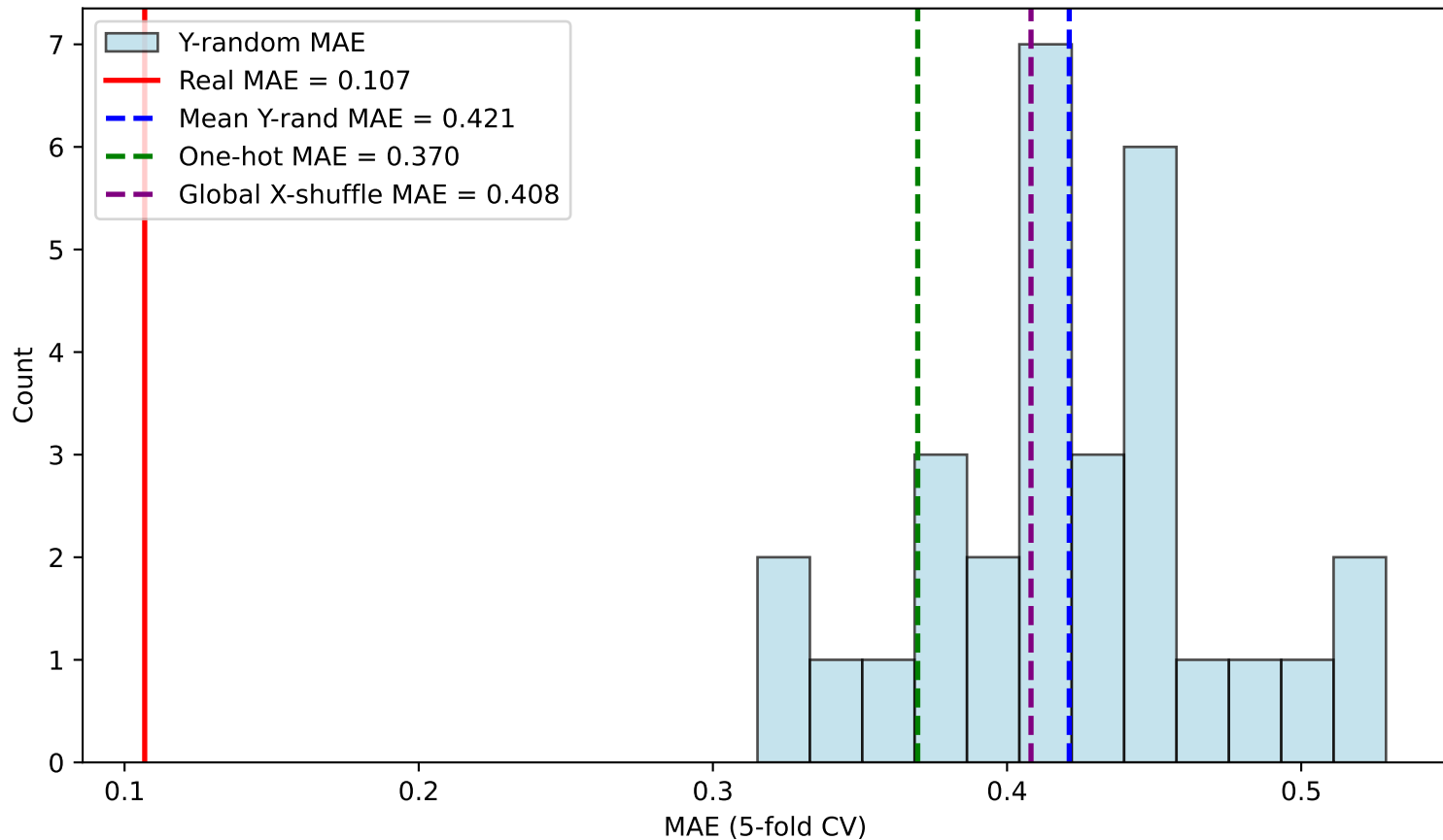
Validation (lower is better): MAE
