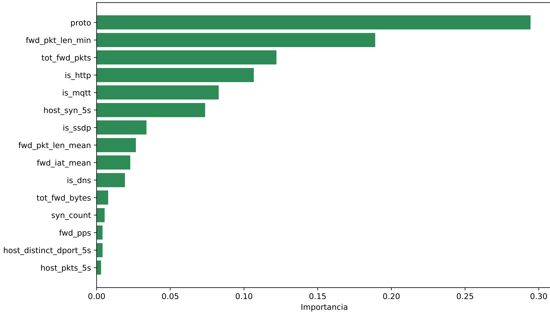
Top-15 features — xgb
