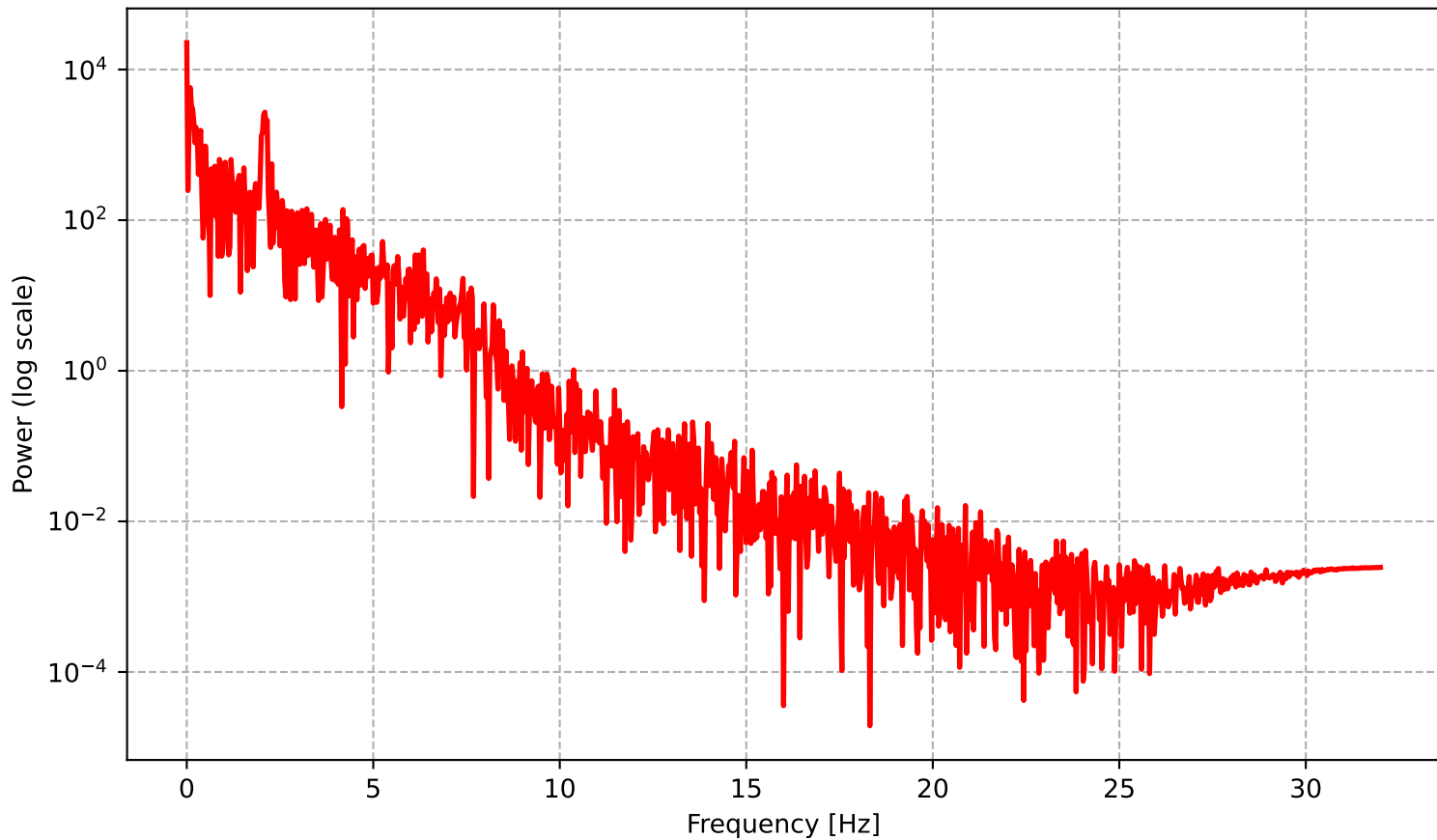
FFT Power Spectrum (ROI 1)
