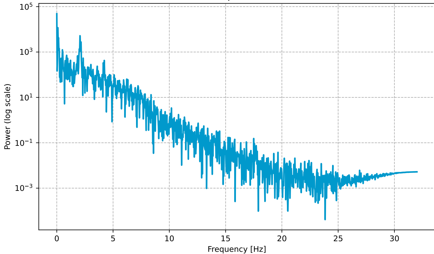
FFT Power Spectrum (ROI 6)
