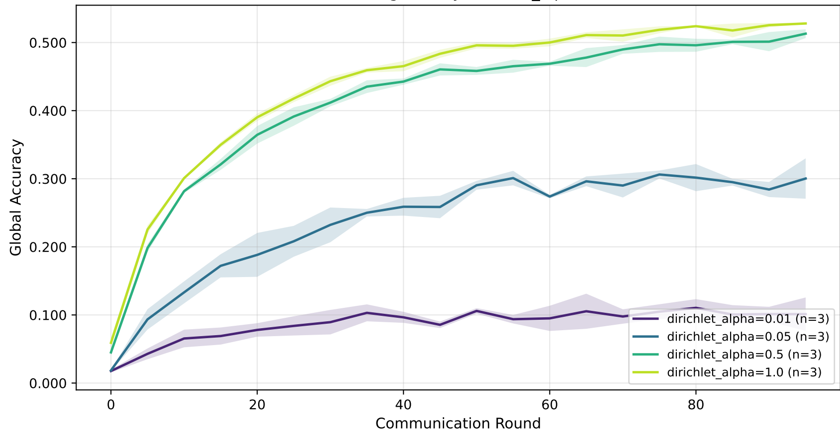
Convergence by dirichlet_alpha
