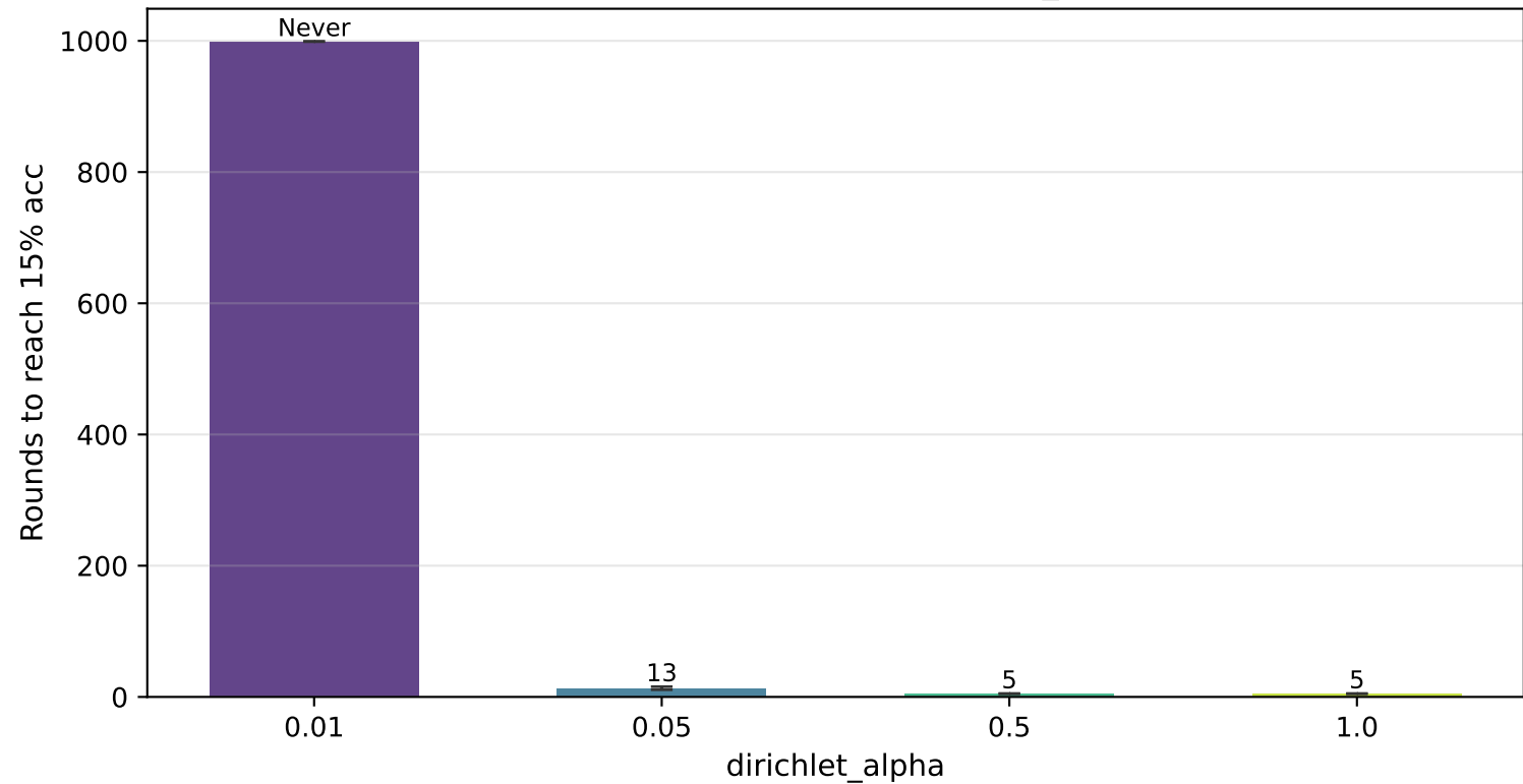
Convergence Speed by dirichlet_alpha
