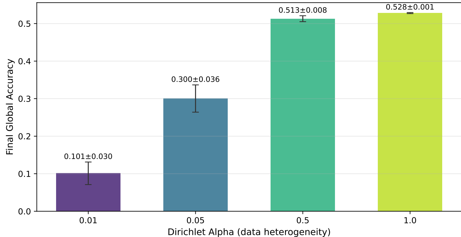
Effect of Data Heterogeneity on Final Accuracy
