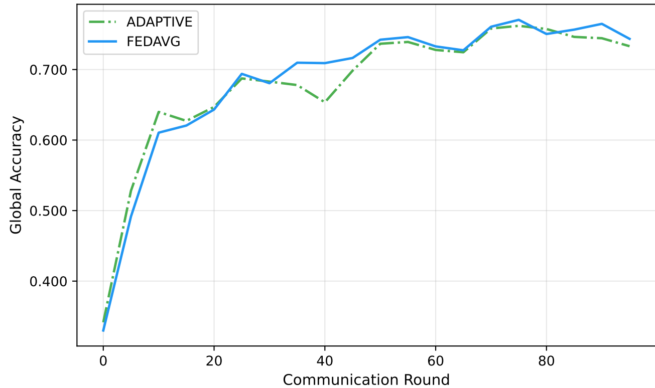
Convergence Under Client Churn
