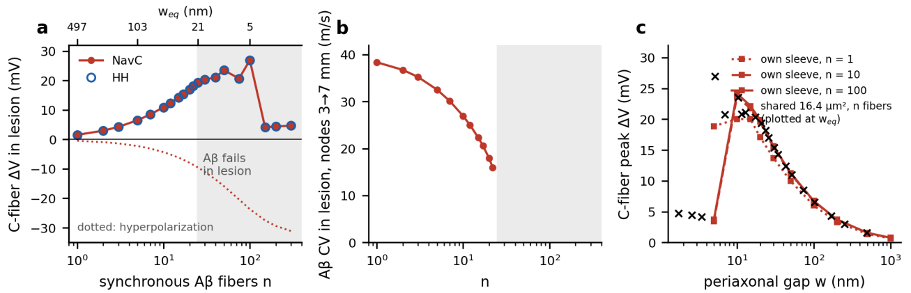
Fig. 5 Synchronous volleys. (a) Peak C-fiber depolarization (solid) and hyperpolarization (dotted) in the lesion vs the number of synchronous A \beta fibers n sharing the 16.4- \mu m^2 compartment; numbers above give the equivalent periaxonal gap w_{eq} ; shading: A \beta conduction fails inside the lesion. (b) A \beta conduction velocity between the 3- and 7-mm nodes. (c) Per-fiber-sleeve closure: response vs sleeve width for n = 1, 10, 100 (NavC), with the shared-compartment results plotted at w_{eq}(n) (crosses).
