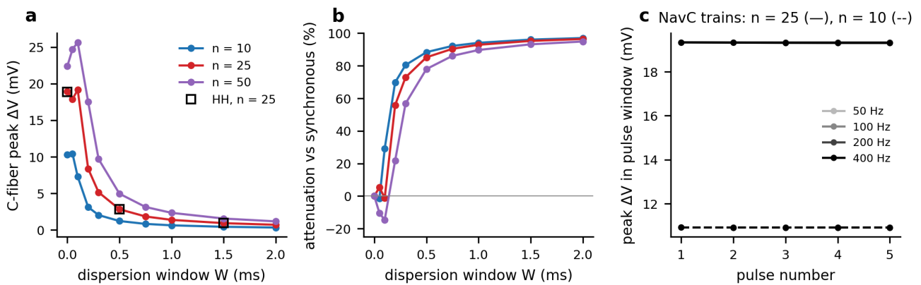
Fig. 8 Temporal dispersion and trains. (a) Peak C-fiber depolarization vs the width W of the onset-dispersion window (NavC; open squares: HH check at n = 25 ). (b) Attenuation relative to the synchronous volley. (c) Per-pulse peak depolarization in 5-pulse trains at 50–400 Hz (NavC).
