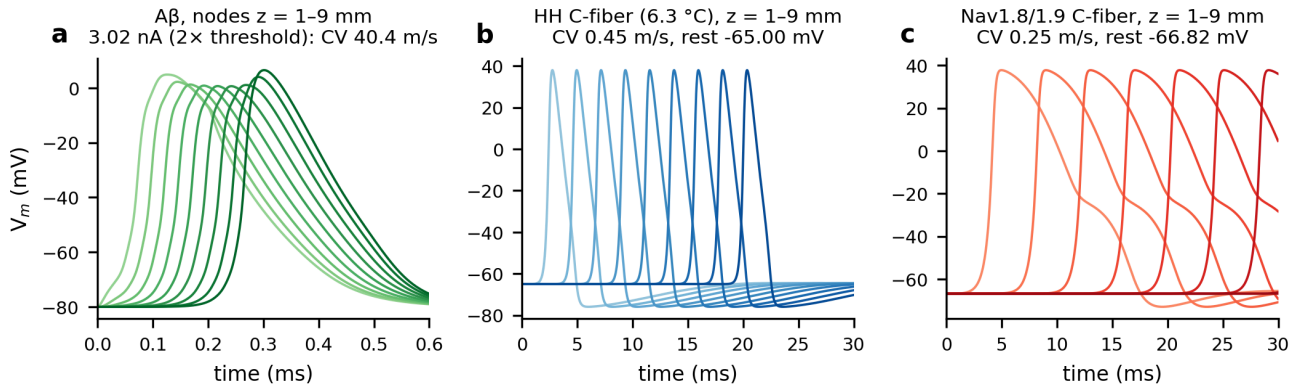
Fig. 3 Uncoupled positive controls. (a) Aβ action potential at nodes z = 1-9 mm (2× threshold stimulus at node 0). (b) HH and (c) NavC C-fiber action potentials at z = 1-9 mm after direct stimulation at z = 0 .
