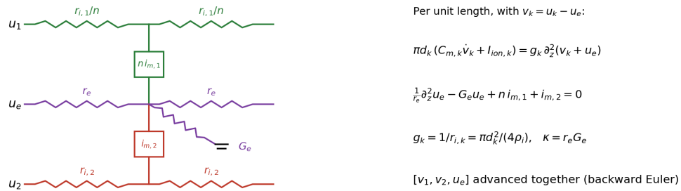
Fig. 1 Model. (a) Geometry: n synchronously stimulated A \beta fibers (CRRSS nodes every 1 mm) and one C-fiber share an extracellular compartment of cross-section A_e along a 5-mm focal lesion; outside the lesion the fibers lie in grounded bulk fluid. The A \beta stimulus ( 2\times threshold, 0.2 ms) is applied at node 0, outside the lesion. (b) Equivalent circuit per unit length and governing equations; the three fields are advanced together.
