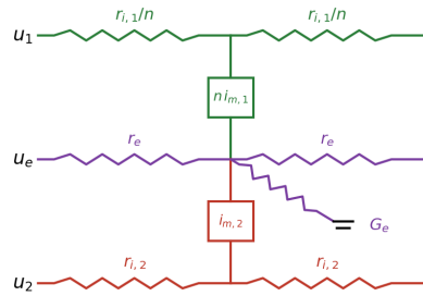
Fig. 1 Model. (a) Geometry: n synchronously stimulated A \beta fibers (CRRSS nodes every 1 mm) and one C-fiber share an extracellular compartment of cross-section A_e along a 5-mm focal lesion; outside the lesion the fibers lie in grounded bulk fluid. The A \beta stimulus ( 2\times threshold, 0.2 ms) is applied at node 0, outside the lesion. (b) Equivalent circuit per unit length and governing equations; the three fields are advanced together.
