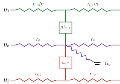
Fig. 1 Model. (a) Geometry: n synchronously stimulated Aβ fibers (CRRSS nodes every 1 mm) and one C-fiber share an extracellular compartment of cross-section A_e along a 5-mm focal lesion; outside the lesion the fibers lie in grounded bulk fluid. The Aβ stimulus ( 2 \times threshold, 0.2 ms) is applied at node 0, outside the lesion. (b) Equivalent circuit per unit length and governing equations; the three fields are advanced together.
