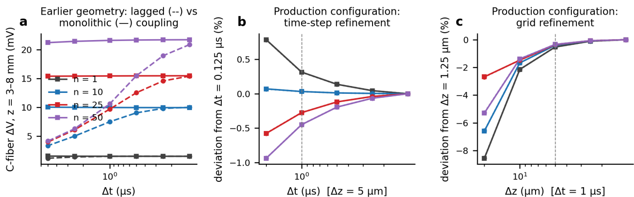
Fig. 2 Numerical verification. (a) Earlier full-length geometry and parameters: C-fiber depolarization vs time step for the lagged coupling scheme of the earlier version (dashed) and the monolithic scheme (solid); the lagged error grows with n . (b, c) Production configuration: deviation of the peak C-fiber depolarization from the finest time step (b) and grid (c) for n = 1, 10, 25, 50 (solid: NavC; dotted: HH); dashed lines mark the production values.
