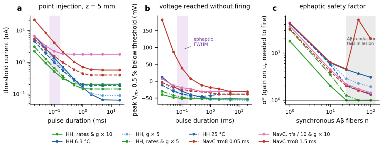
Fig. 6 Excitability of the C-fiber for brief, local inputs. (a) Strength–duration curves for point injection at z = 5 mm; shading marks the duration of the ephaptic depolarization. (b) Membrane potential at the injection site for a pulse 0.5 % below threshold. (c) Ephaptic safety factor \alpha^* , the gain on the recorded u_e needed to evoke a propagating C-fiber AP, vs n ; \alpha^* = 1 (line) would mean that the closed-loop drive itself fires the fiber.
