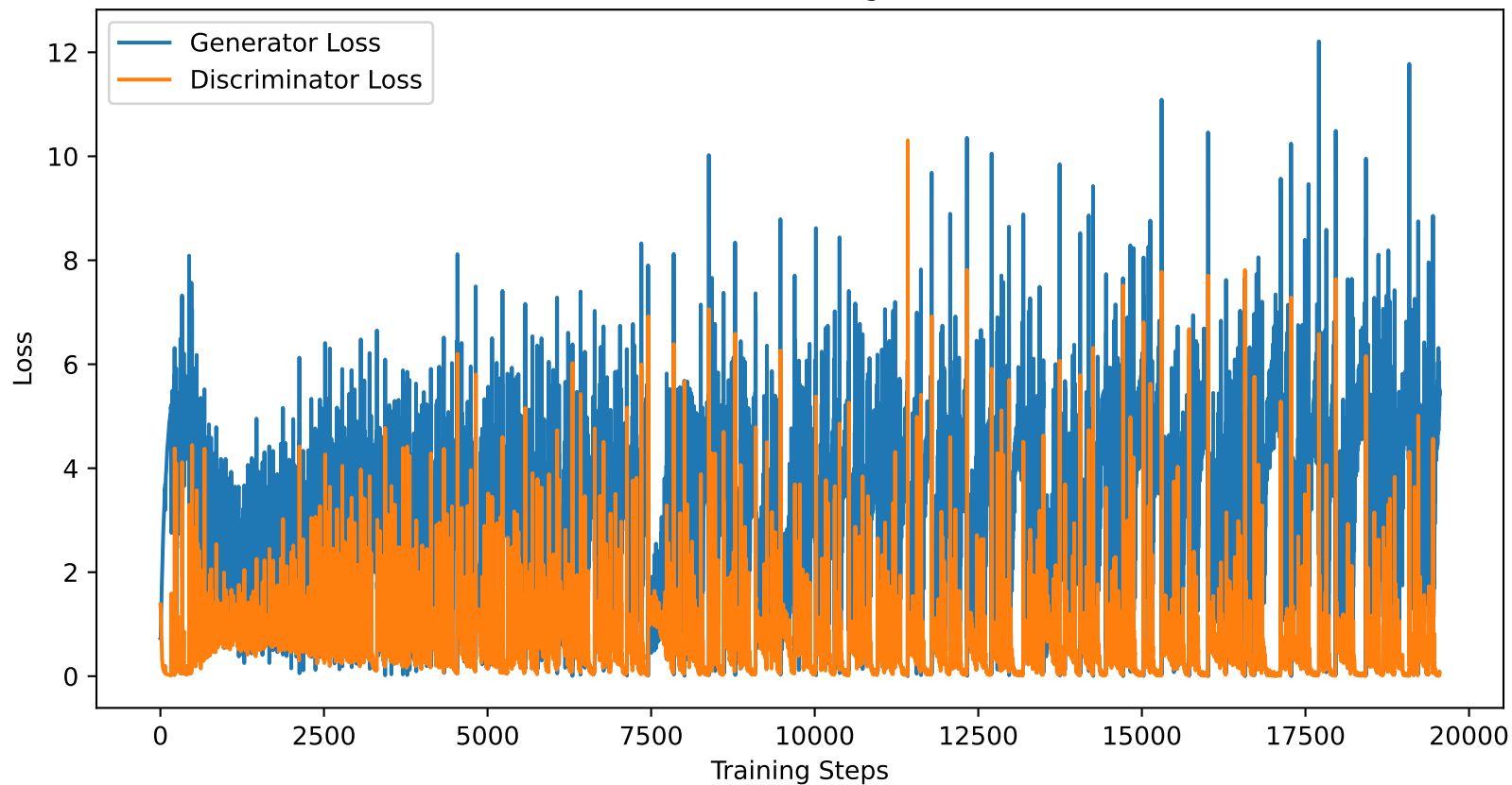
DCGAN Training Loss
