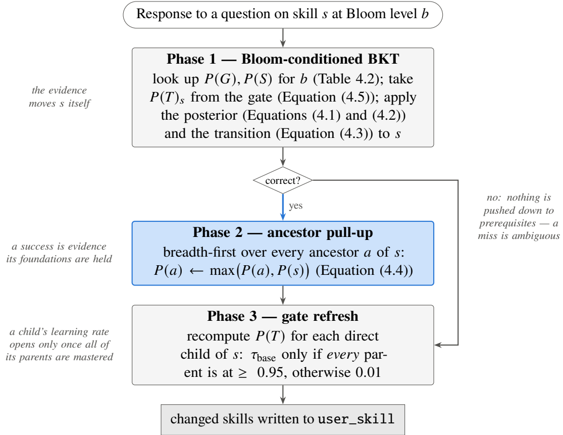
Figure 4.6: The three-phase update that every response triggers. Phase 1 is textbook BKT with Bloom-conditioned noise; Phase 2 lifts every ancestor to at least the answered skill after a success; Phase 3 keeps each child's learning rate in step with its parents. Only correct answers propagate, which is also why a later wrong answer can break the ordering Phase 2 set (Section 5.3.8).
