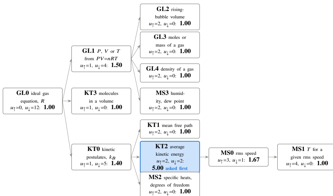
Figure 4.9: Choosing the first diagnostic question in the Ideal Gas and Kinetic Theory section (13 skills, 12 prerequisite edges; GL = gas laws, KT = kinetic theory, MS = molecular speeds). Each skill is scored by Equation (4.6) from its untested ancestors u_\uparrow and descendants u_\downarrow . The root GL0 touches every skill but only from one side (1.00); KT2 sits between two unknown regions of equal size and scores 5.00, so its outcome says the most about both, and the live diagnostic asked it first.
