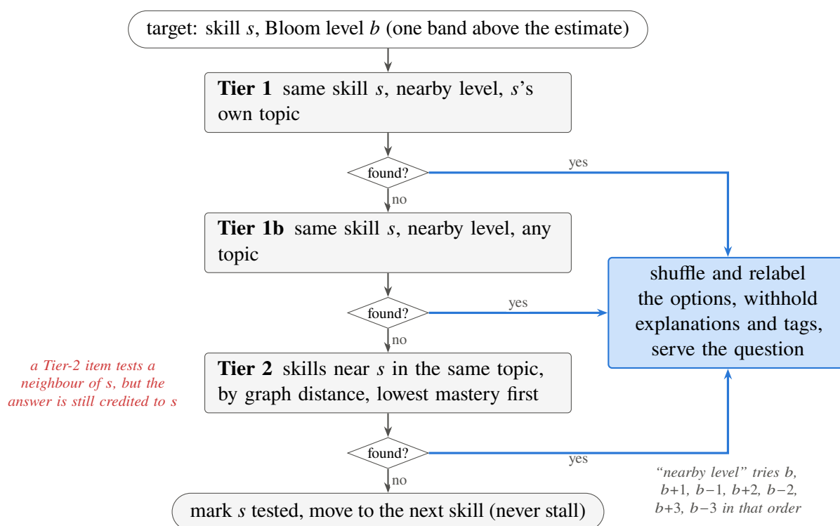
Figure 4.10: The fallback ladder that finds a question for the skill and level the diagnostic has chosen. Each tier widens the search; a skill with nothing to ask is skipped rather than stalling the session. Whatever tier supplies the item, the answer updates the target skill at the target level — the source of the attribution gap measured in Section 5.3.9.
