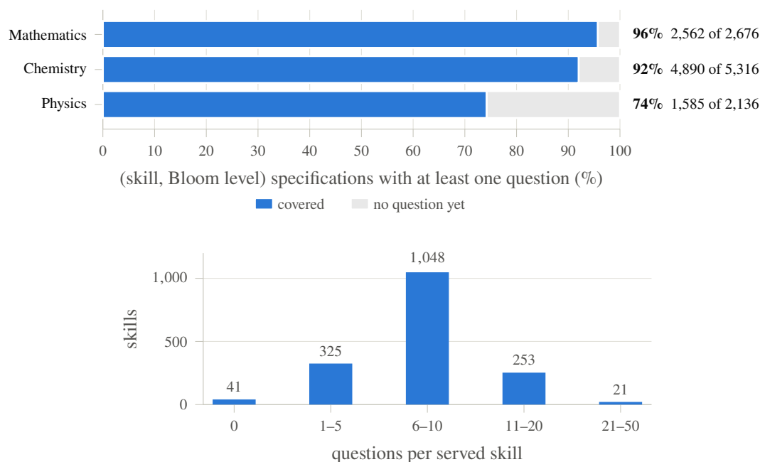
Figure 4.18: The question bank against the served ontology. Top: 9,037 of the 1,688 \times 6 = 10,128 generation specifications (89%) hold at least one verified question; Physics is the thin subject. Bottom: a typical skill has six to ten questions spread over its Bloom levels, and 41 skills (31 of them in Physics) have none, which is what shortens some diagnostics (Section 5.3.10). A further 7,692 questions in the database are keyed to 487 legacy skill identifiers and are unreachable by the engine.
