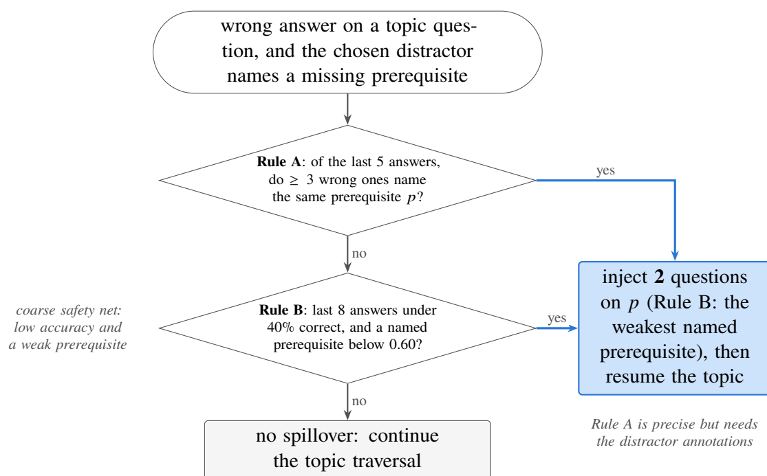
Figure 4.11: Prerequisite spillover during topic practice. Every distractor in the bank is annotated with the skill whose absence would lead a learner to choose it ( option_missing_prerequisites ); Rule A acts on that evidence directly, Rule B on accuracy and mastery. Spillover is considered only after a wrong answer whose distractor carries such a tag and only when no spillover is already running. Figure 5.3 shows Rule A firing in a live session.
