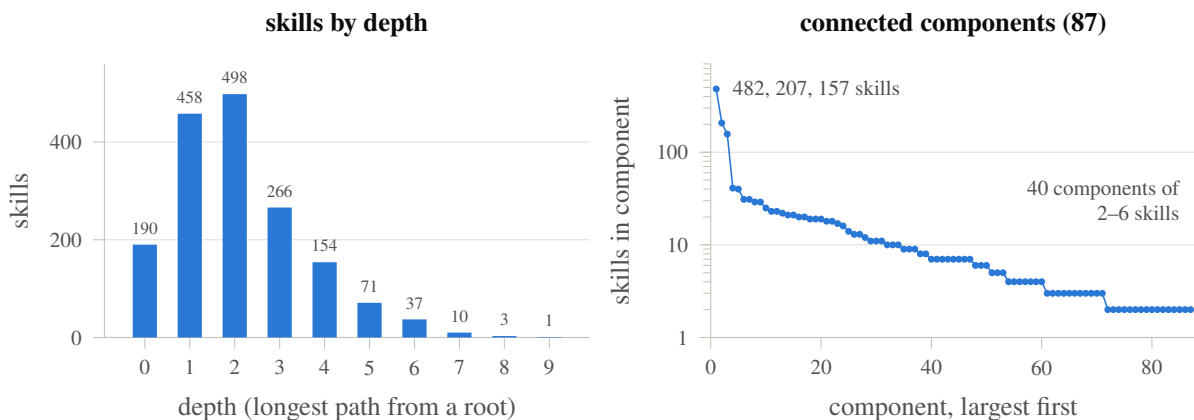
Figure 4.14: Shape of the served skill graph (1,688 skills, 1,683 direct edges). Left: most skills sit one to three prerequisites deep; the deepest chain has nine. Right: the graph is not one piece. Three large components hold 846 skills between them, and the long tail of small fragments is where a missing edge most often goes unnoticed. Of the 40 components of 2–6 skills, 32 are the near-orphan fragments of Table 5.1 still awaiting a domain expert (Section 5.1); the other 8 share their topic with no lower-tier skill outside themselves, so there is nothing within the topic to attach them to.
