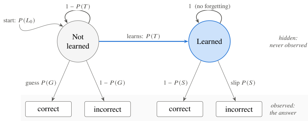
Figure 4.3: Bayesian Knowledge Tracing as a two-state hidden Markov model. The engine never sees which state a learner is in, only the answers, so it keeps P(L) , the probability of the Learned state, and revises it with Equations (4.1) to (4.3) after every response. Guess and slip are what make a single answer weak evidence: a right answer may be a guess, and a wrong one may be a slip.
