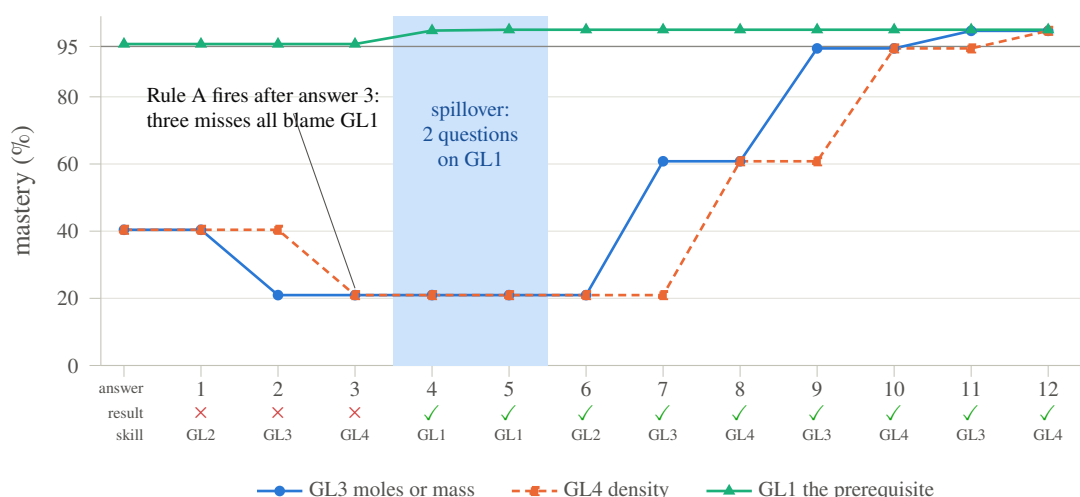
Figure 5.3: Topic practice on Ideal Gas Laws after the diagnostic of Figure 5.2, against the live bank. The first three answers are wrong, and every distractor chosen names GL1 as the missing prerequisite, so spillover Rule A fires and injects two GL1 questions (shaded) — although GL1 was already estimated at 96%, since Rule A does not consult the prerequisite's own estimate (Rule B does). Practice then returns to the topic and cycles through the skills still below the 95% threshold (grey line); each correct answer moves one skill by one Bloom-conditioned update. The session ends by itself after twelve answers, when all five topic skills pass the threshold (GL0 and GL2, already above it, are not plotted).
