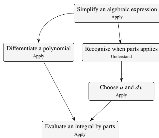
Figure 4.12: A fragment of the skill graph, illustrating the granularity target. “Integration by parts” is not one node but a chain: recognising applicability, choosing the decomposition, and executing it — each separately testable, and each with its own prerequisites, so that a failure can be localised to the step that actually broke.
