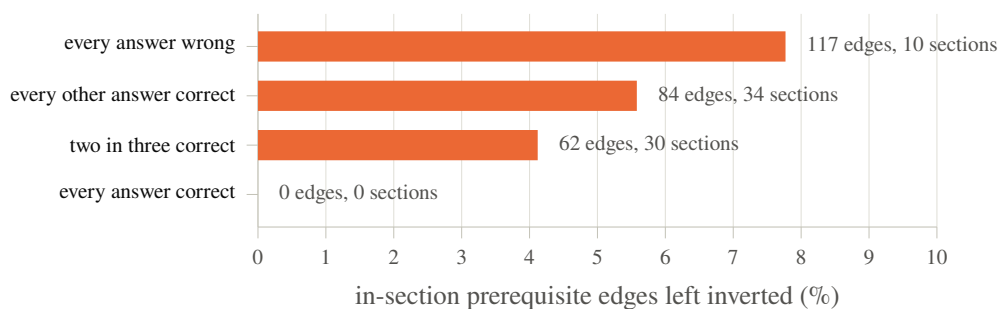
Figure 5.6: How often the ordering “no ancestor below its descendant” survives a diagnostic, over all 51 sections (1,505 in-section edges) for four answer patterns. With only correct answers it always holds, because pull-up runs after every success. A wrong answer lowers only the answered skill: if a descendant already sits higher — credited by an earlier correct answer, or simply still at its depth-based prior — the order is broken, and nothing restores it (Section 5.3.8).
