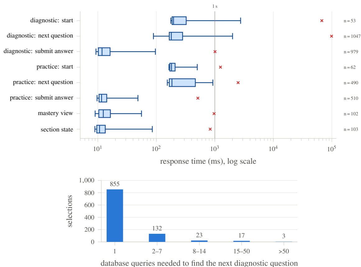
Figure 5.4: Responsiveness (NFR2), measured over 4,862 requests of the live end-to-end run. Top: boxes span the 25th–75th percentile with the median marked; whiskers reach the 5th and 95th; × is the slowest call. Answer submission is fast (median about 12 ms); choosing a new question has a median near 180 ms but a long tail. Bottom: the tail comes from the fallback ladder, counted by replaying the same code over a copy of the bank. 855 of 1,030 selections need a single query, but where the bank is thin the ladder issues one query per candidate (skill, level) pair, up to 100, and each is a round trip to the hosted database.
