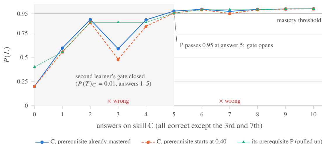
Figure 4.8: The conjunctive gate in practice, computed by the engine. Two learners give the same answers on a skill C whose one prerequisite P is either already mastered (gate open, P(T)_C = 0.10 ) or starts at 0.40 (gate closed, P(T)_C = 0.01 ). The Bayesian evidence dominates: the closed-gate learner trails by at most 0.11. Each correct answer on C also pulls P up to C's value, so P crosses 0.95 at the fifth answer and the gate opens. The gate therefore withholds only the unobserved learning credit; the ordering between a skill and its prerequisites comes from pull-up.
