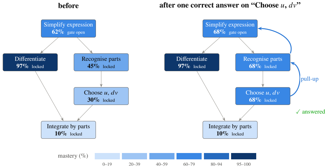
Figure 4.7: The policy on the skill fragment of Figure 4.12. One correct answer on “Choose u and dv ” raises it from 30% to 68% (Phase 1; its gate is locked because “Recognise parts” is below 95%, so it learns at 0.01). Phase 2 then lifts both of its ancestors to the same 68%. “Integrate by parts” is untouched: pull-up never flows downward, and its gate stays locked until both of its parents reach 95%.
