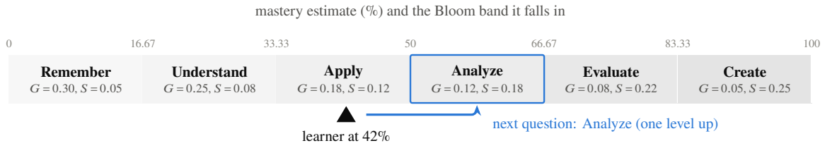
Figure 4.4: The 0–100 mastery scale is cut into six equal bands, one per Bloom level, each with its own guess and slip values (Table 4.2). The selection rule reads the band a learner is in and asks one level above it, capped at Create: a learner estimated at 42% sits in Apply, so the next question is an Analyze item.
