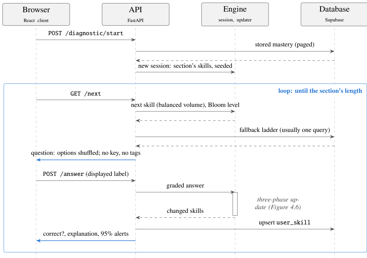
Figure 4.16: One diagnostic, request by request. Sessions live in the API process; only mastery is persisted. The answer key never leaves the server before the learner answers: options are shuffled when a question is first served, the shuffled copy is kept as the session's current question, and the answer is graded against the label the learner saw.
