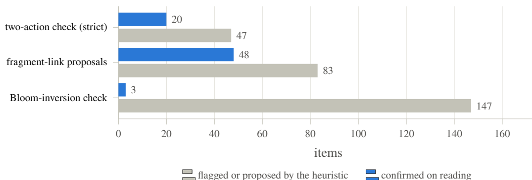
Figure 5.1: Mechanical heuristics against hand review. The Bloom-inversion check was right about 3 of its 147 flags; the strict two-action check about 20 of 47 (its first version flagged 173, over half of them wrongly); edge proposals for disconnected fragments were accepted 48 times in 83, several only after reversing their direction. Every flag was read before anything was changed.
