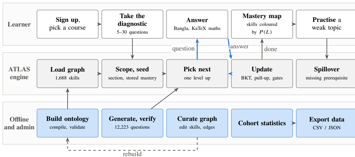
Figure 4.1: The learner’s journey through ATLAS and what the engine and the offline and administrative side do at each step. The blue loop is the core of the system: each answer updates mastery and chooses the next question, until the section’s diagnostic length is reached. Graph edits made by an administrator reach learners only after the ontology is rebuilt (dashed).
