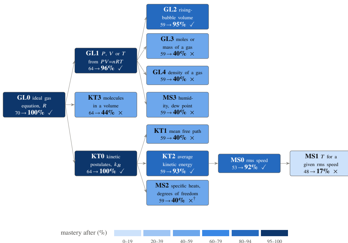
Figure 5.2: The Ideal Gas section after a 13-question diagnostic against the live question bank, answering the first six correctly and the rest wrongly. Each node shows the depth-based prior and the estimate afterwards; ✓ and × mark the answers the engine credited to that skill. The correct answers on KT0 and GL1 lifted the root GL0 to 100% before it was asked (pull-up), while the wrong answers left their own skills near 40%. † MS2 has no question in the bank at the requested level, so the fallback ladder served an MS0 item in its place and the answer was credited to MS2 (Section 5.3.9).
