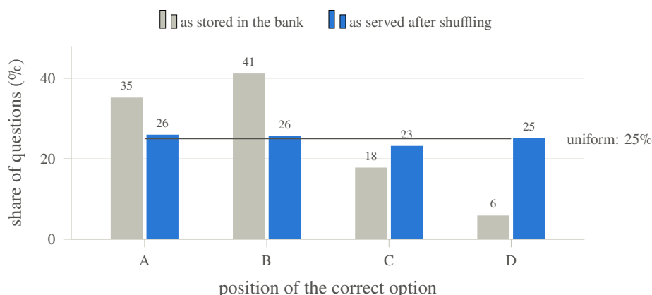
Figure 5.5: Where the correct answer sits. In the bank, the key is A or B in 76% of questions and D in only 6%, so a learner who always picked B would score 41% without reading a question. Options are now shuffled when a question is served (Section 5.3.7); across the 1,489 questions served in the live run the key’s position is close to uniform.
