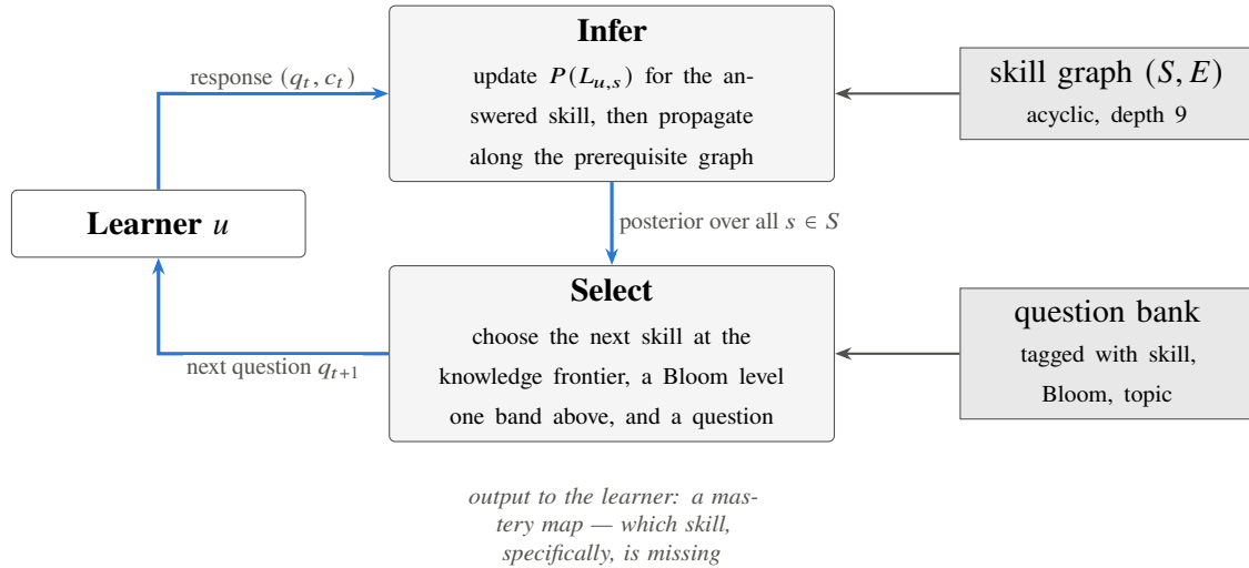
Figure 1.2: The problem as a closed loop. Each response is weak, noisy evidence about one skill; the inference step turns it into a posterior over every skill in the graph, and the selection step spends the next question where that posterior is least certain. The two stores are the fixed inputs defined in Section 1.2.
