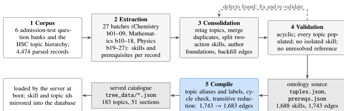
Figure 4.13: How the skill graph was built. Stages 1–4 produced the ontology source offline; stage 5 is a one-command, reproducible compile, so the served catalogue is never edited by hand. Transitive reduction removes the 60 edges already implied by a longer path, which the conjunctive gate (Equation (4.5)) requires.
