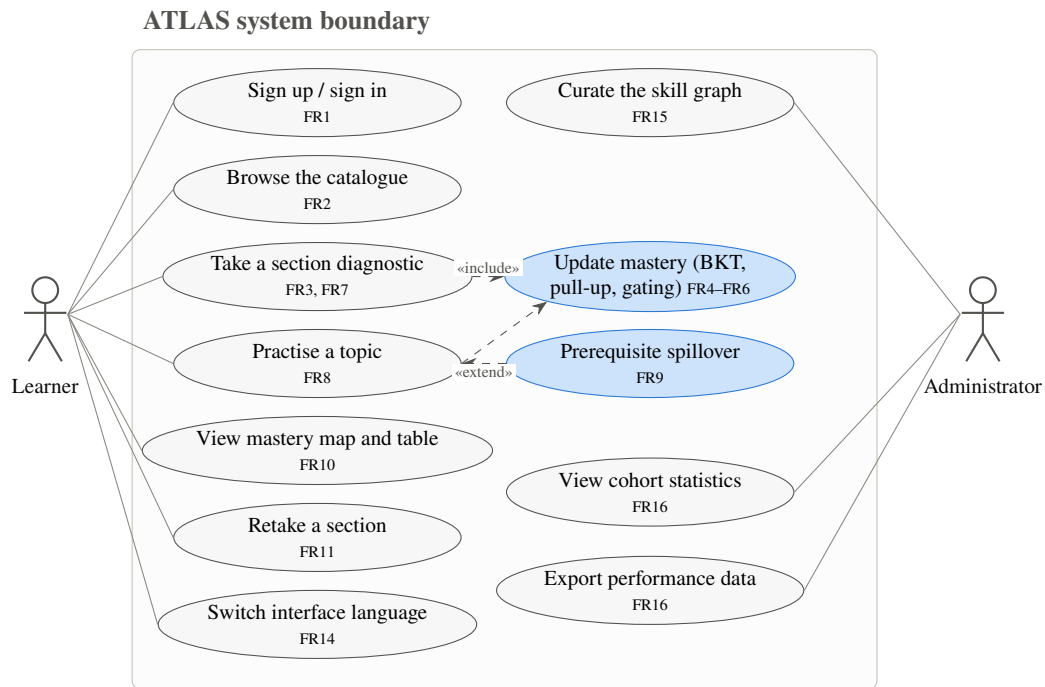
Figure 3.1: Use cases, labelled with the functional requirements of Table 3.2 they realise. The shaded cases are not requested by the learner directly: every diagnostic and practice answer triggers the mastery update, and spillover extends practice when repeated failure points at a missing prerequisite. The administrator cases were added late in the project (FR15, FR16).
