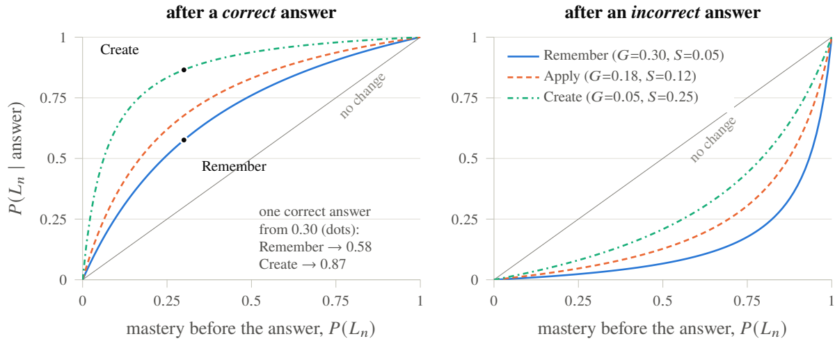
Figure 4.5: How far one answer moves the estimate depends on the question’s Bloom level (Equations (4.1) and (4.2), parameters from Table 4.2; the learning transition is omitted to isolate the effect). A correct answer on a Create item is strong evidence because it is hard to guess; the same answer on a Remember item is weaker because nearly a third of non-knowers ( P(G) = 0.30 ) would pick it anyway. Wrong answers show the mirror image: a miss on a Create item is partly forgiven as a slip.
