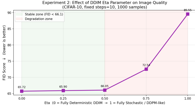
Fig. 7. FID vs. eta at fixed 10 steps. Green zone (eta 0.0 to 0.5): stable region with under 0.5 percent FID change. Red zone (eta 0.5 to 1.0): sharp degradation where FID rises from 66.05 to 89.55. The phase transition at eta 0.5 is an original empirical finding of this work.
