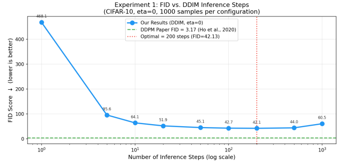
Fig. 6. FID vs. DDIM inference steps (log x-axis). Optimal at 200 steps (FID 42.13) marked by red dotted line. The green dashed line shows the paper-reported FID of 3.17. FID degrades at both extremes due to insufficient denoising (left) and ODE discretization error accumulation (right).
