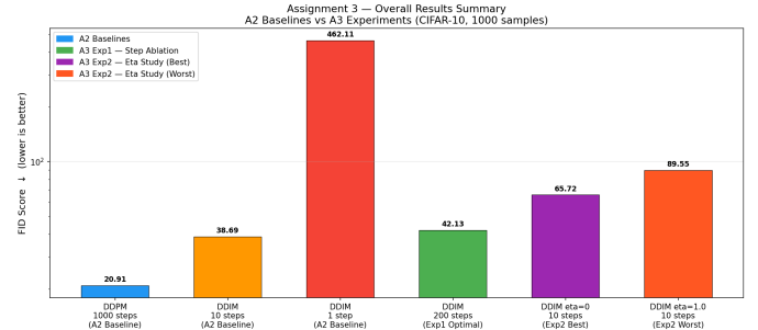
Fig. 9. Comprehensive FID comparison across all A2 baselines and A3 experiments on CIFAR-10 (log scale). The optimal A3 DDIM-200 (FID 42.13) is competitive with A2 DDIM-10 (FID 38.69) but does not surpass full DDPM-1000 stochastic sampling (FID 20.91), confirming that inference optimization reduces but does not eliminate the gap.
