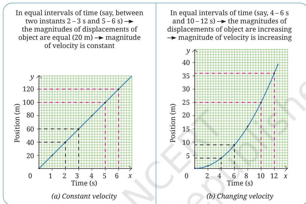
Fig. 4.13: Position-time graph of a moving object
