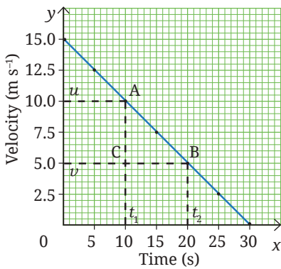
Fig. 4.17(e): Calculating acceleration from a velocity-time graph
