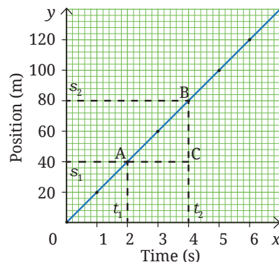
Fig. 4.14: Calculating velocity from a position-time graph
