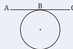
Fig. 4.25: Tangent to a circle at point B
