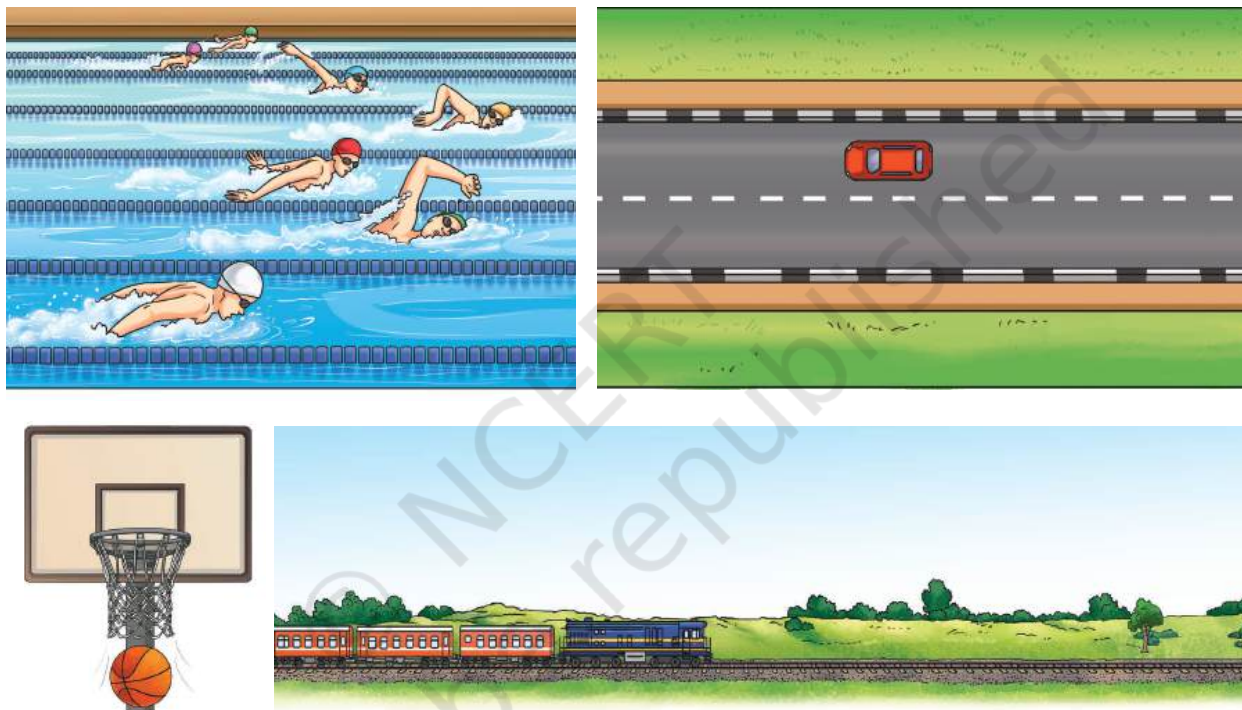
Fig. 4.1: Objects in a straight line motion
