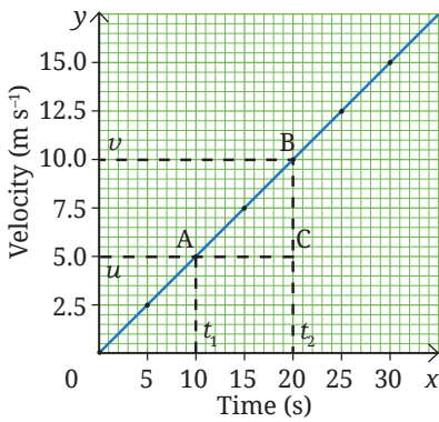
Fig. 4.17(d): Calculating acceleration from a velocity-time graph
