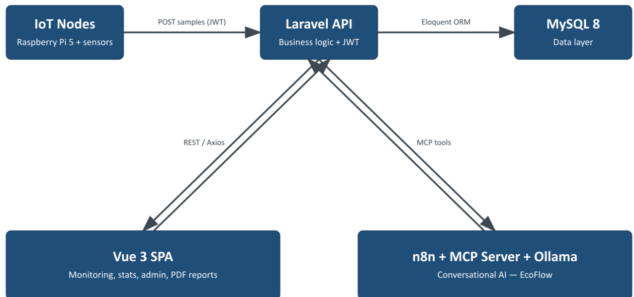
Fig. 1.1. SMMyE five-layer system architecture
