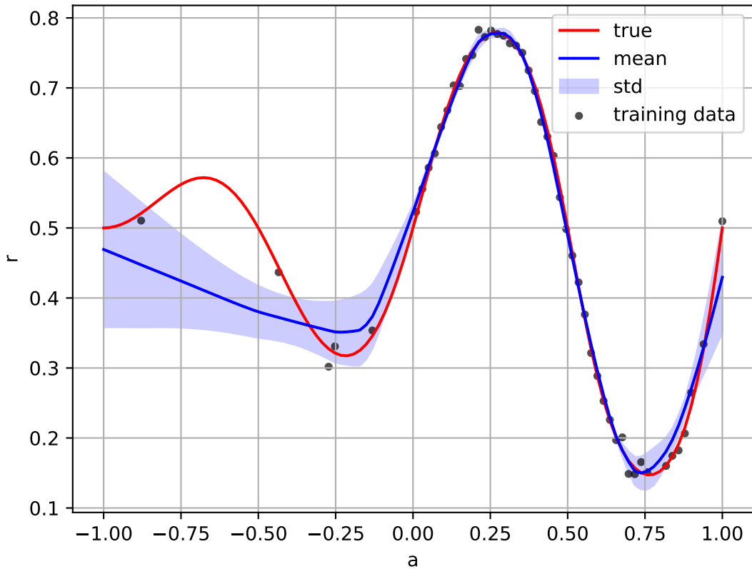
Bootstrapping with k=10 , n=50
