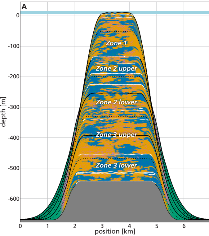
sediment profile
