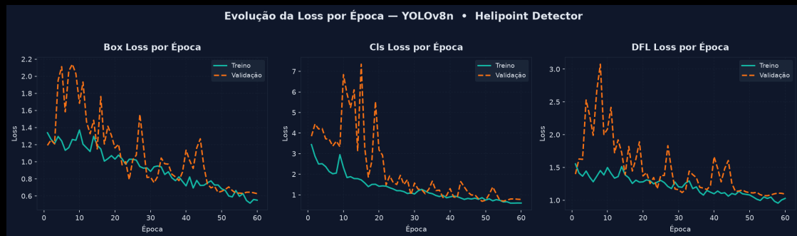
Figure 1 — Evolution of the losses (Box, Cls, DFL) per epoch, train vs. validation. No clear sign of overfitting across the 60 epochs; val/cl s _loss oscillates in the first 20 epochs and stabilizes from epoch 30 onward.
