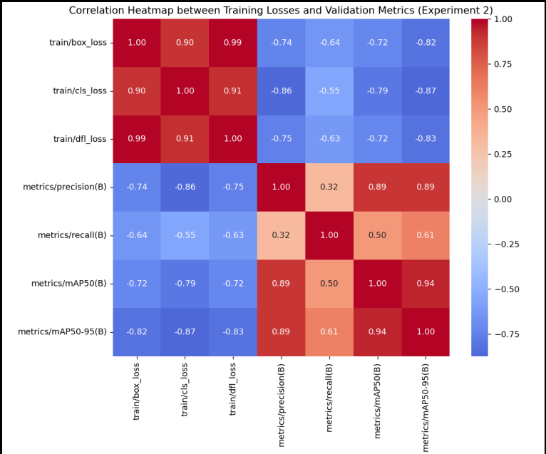
Correlation between training losses and validation metrics (exp2).
