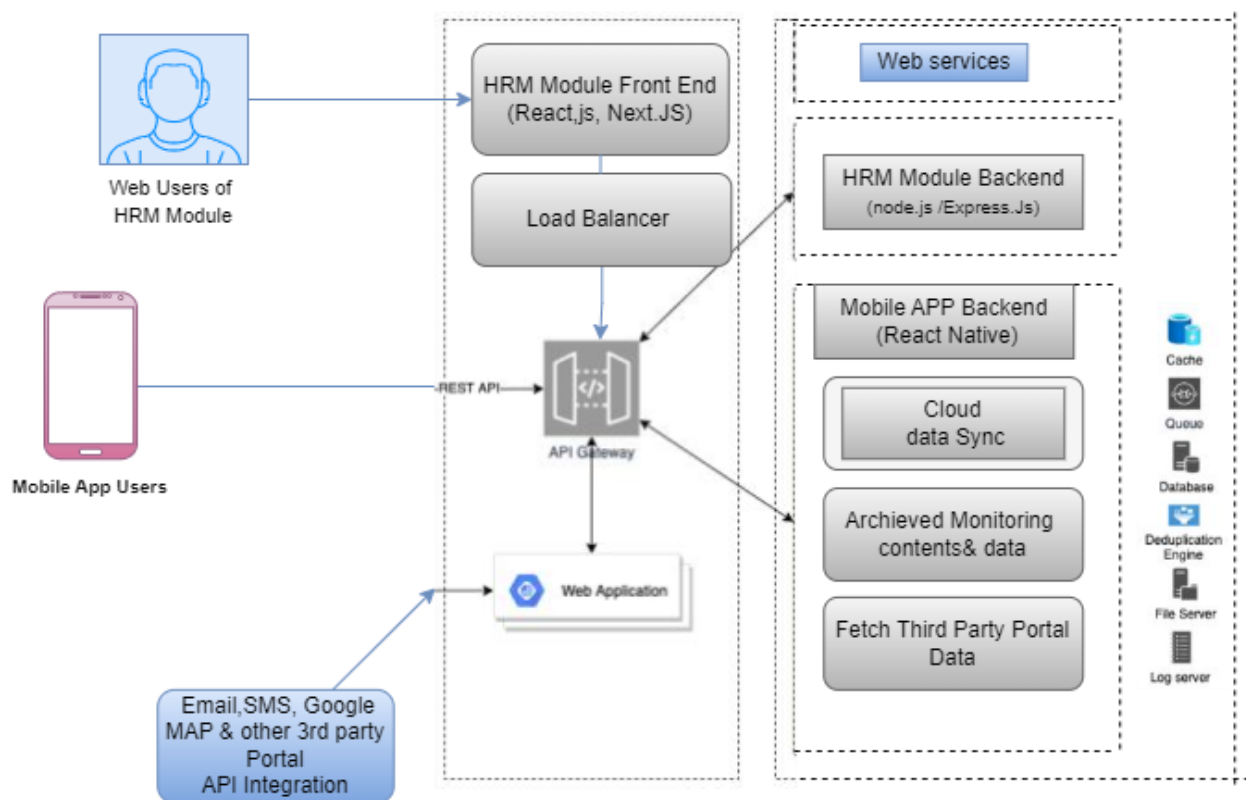
System Architecture of ASF ERP System (HRM Module)
